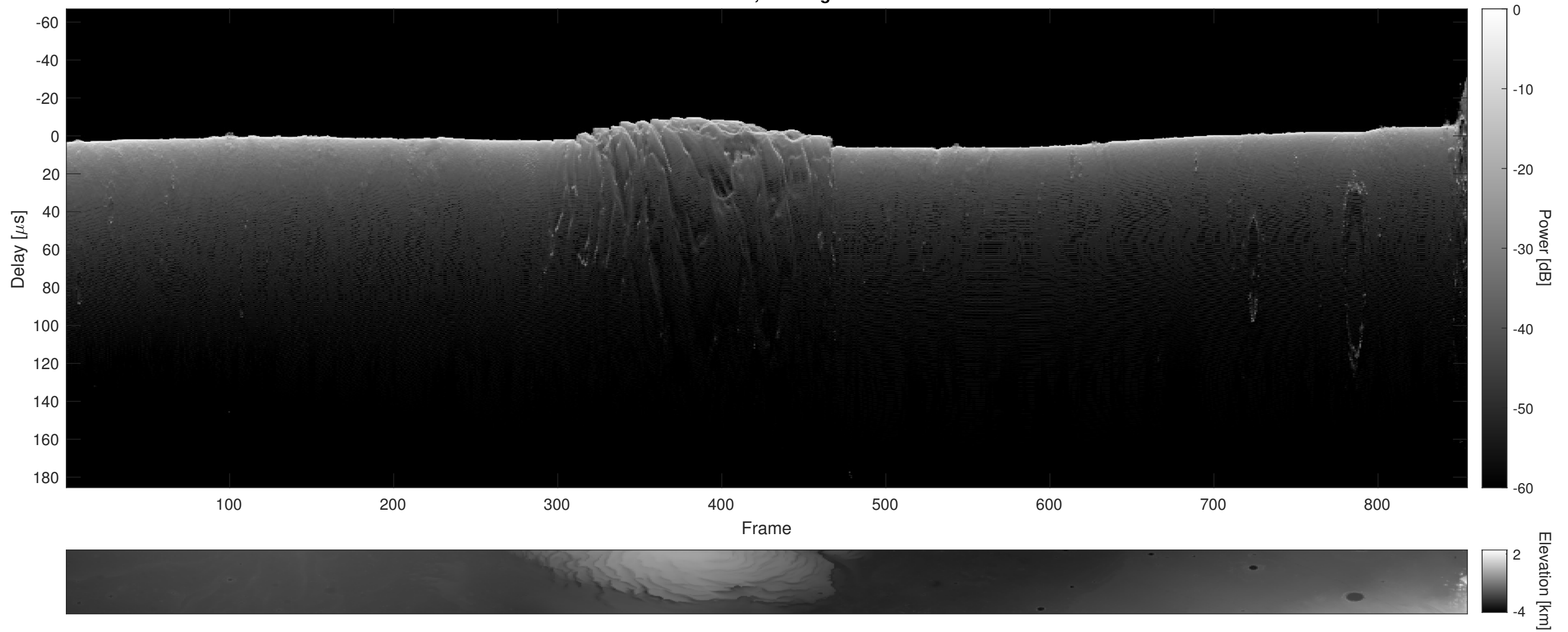
Orbit 9668, Cluttergram
