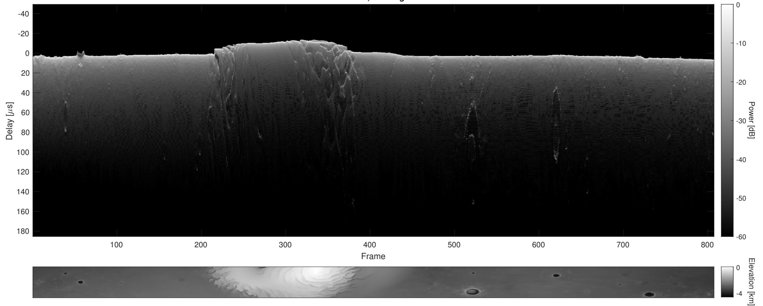
Orbit 9669, Cluttergram
