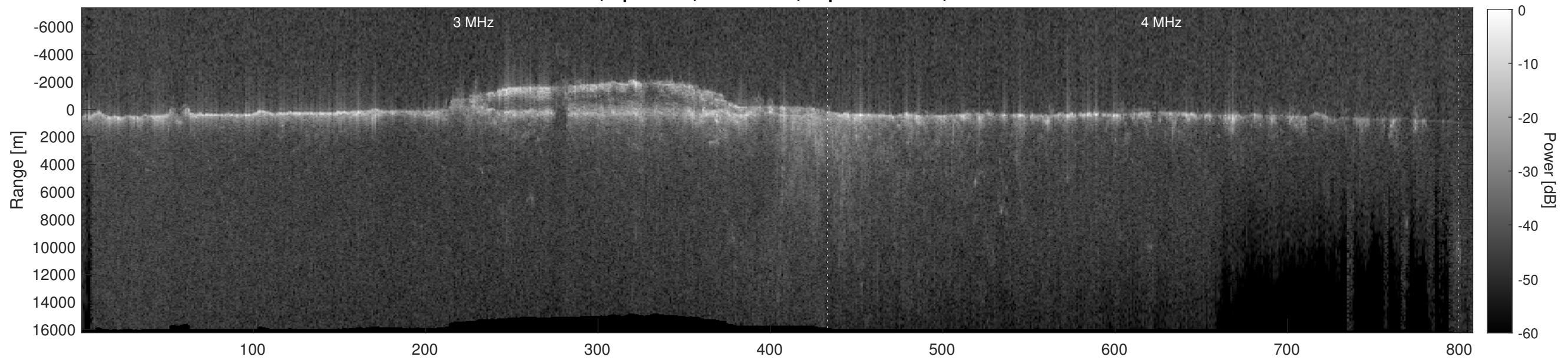
Orbit 9669, Depth-Corrected Cluttergram
