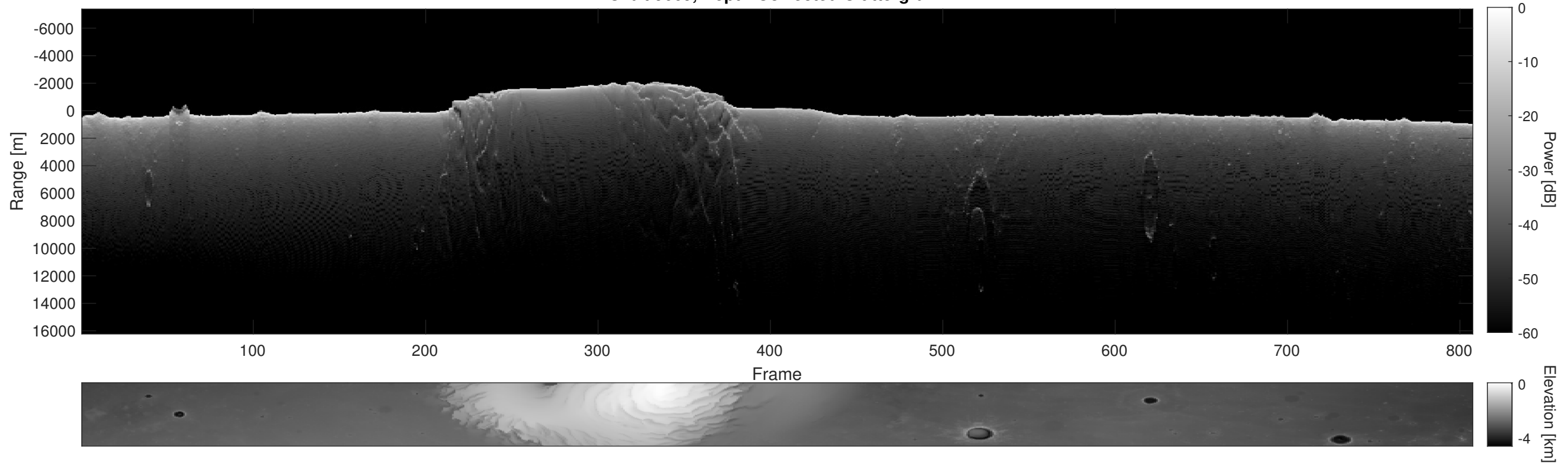
Orbit 9669, Depth-Corrected Cluttergram
