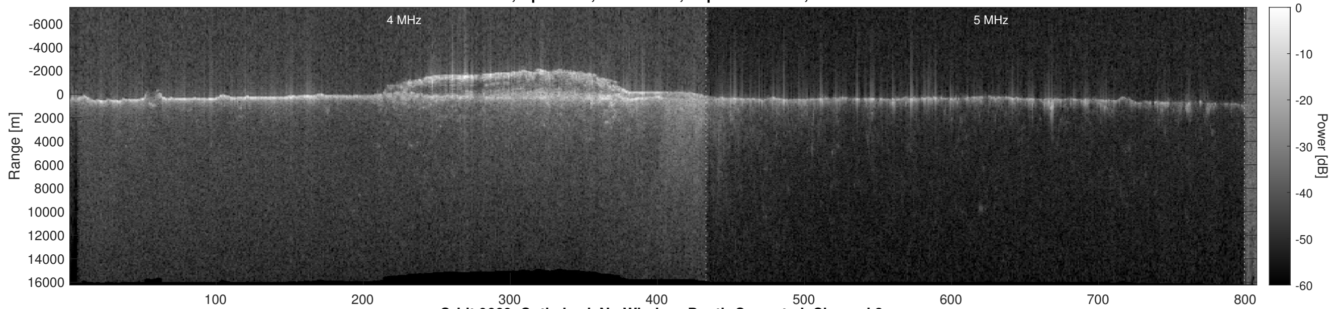
Orbit 9669, Optimized, No Window, Depth-Corrected, Channel 2
