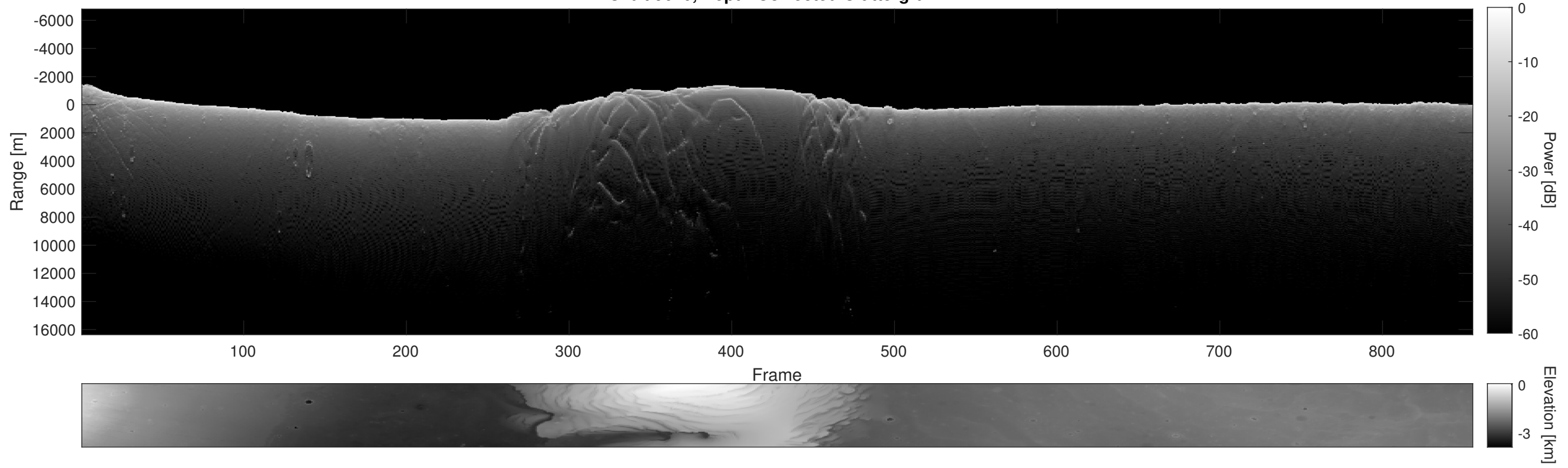
Orbit 9670, Depth-Corrected Cluttergram
