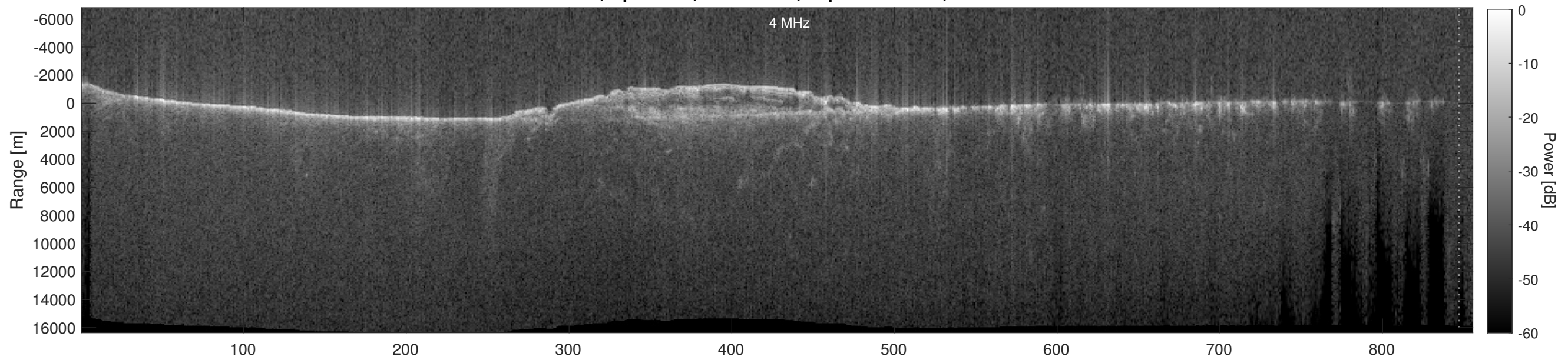
Orbit 9670, Depth-Corrected Cluttergram
