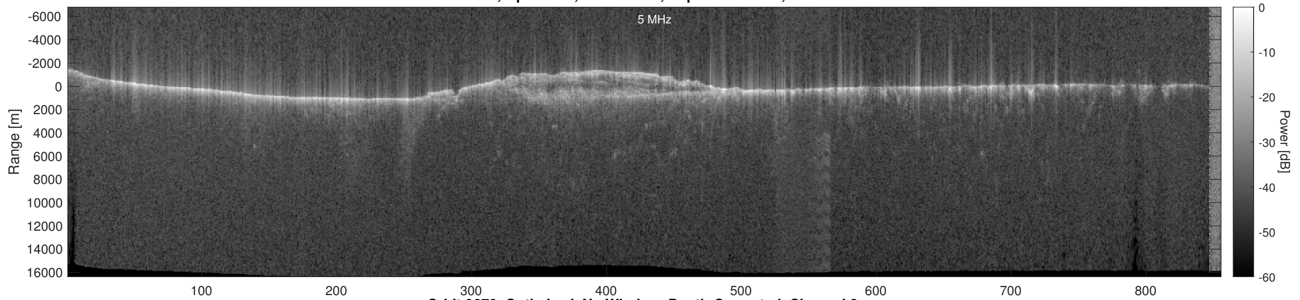
Orbit 9670, Optimized, No Window, Depth-Corrected, Channel 2
