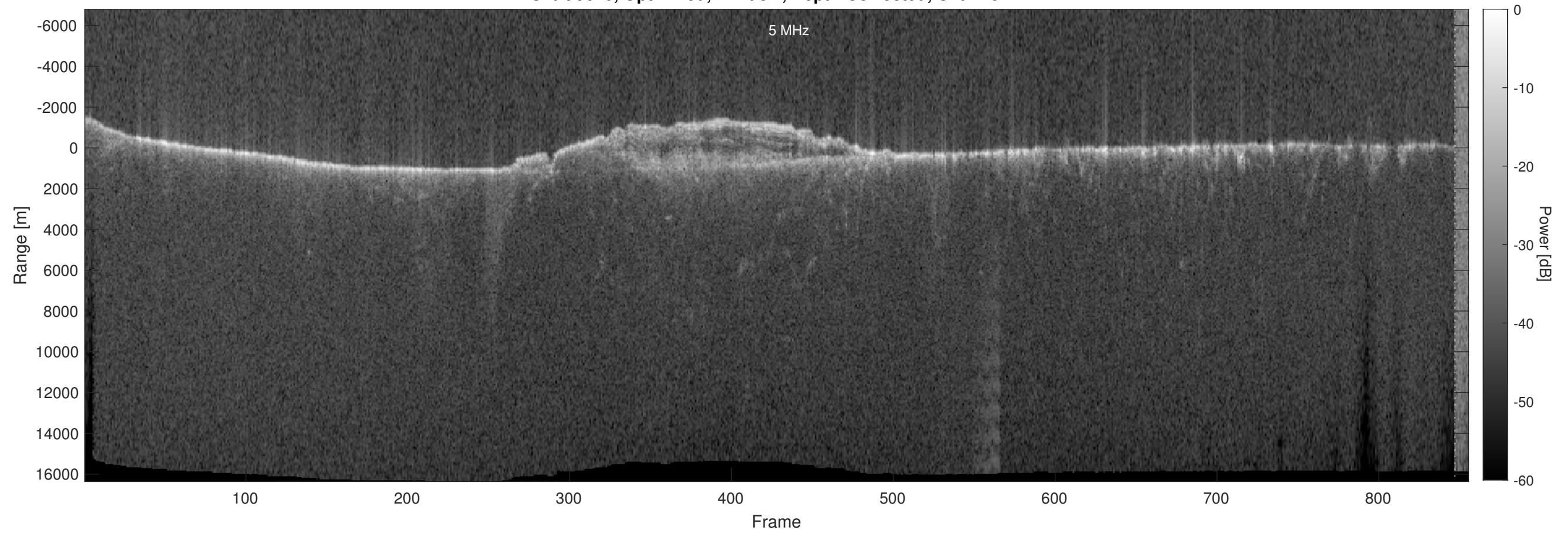
Orbit 9670, Optimized, Window, Depth-Corrected, Channel 2
