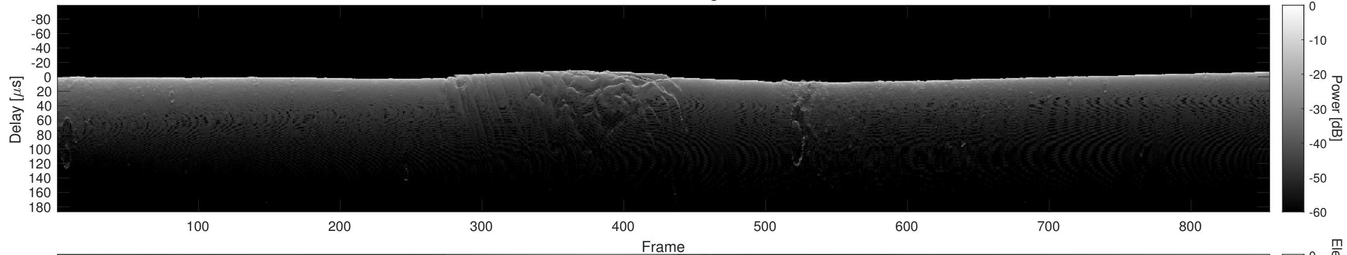
Orbit 9672, Cluttergram
