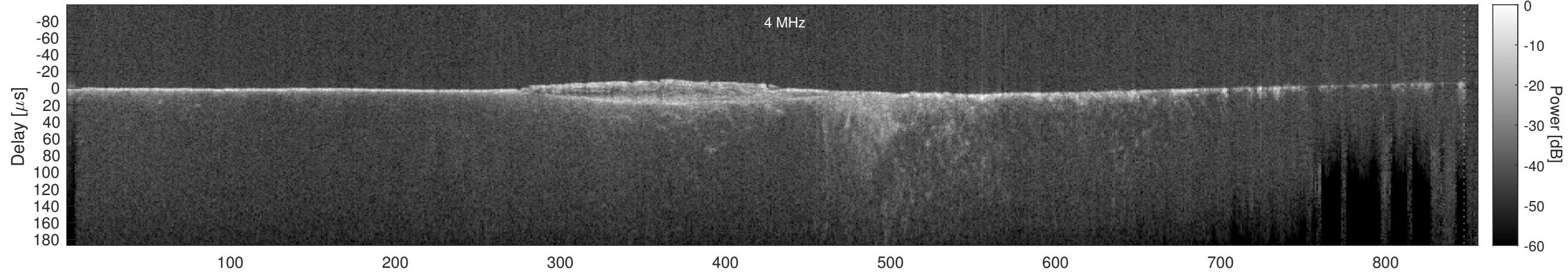
Orbit 9672, Cluttergram
