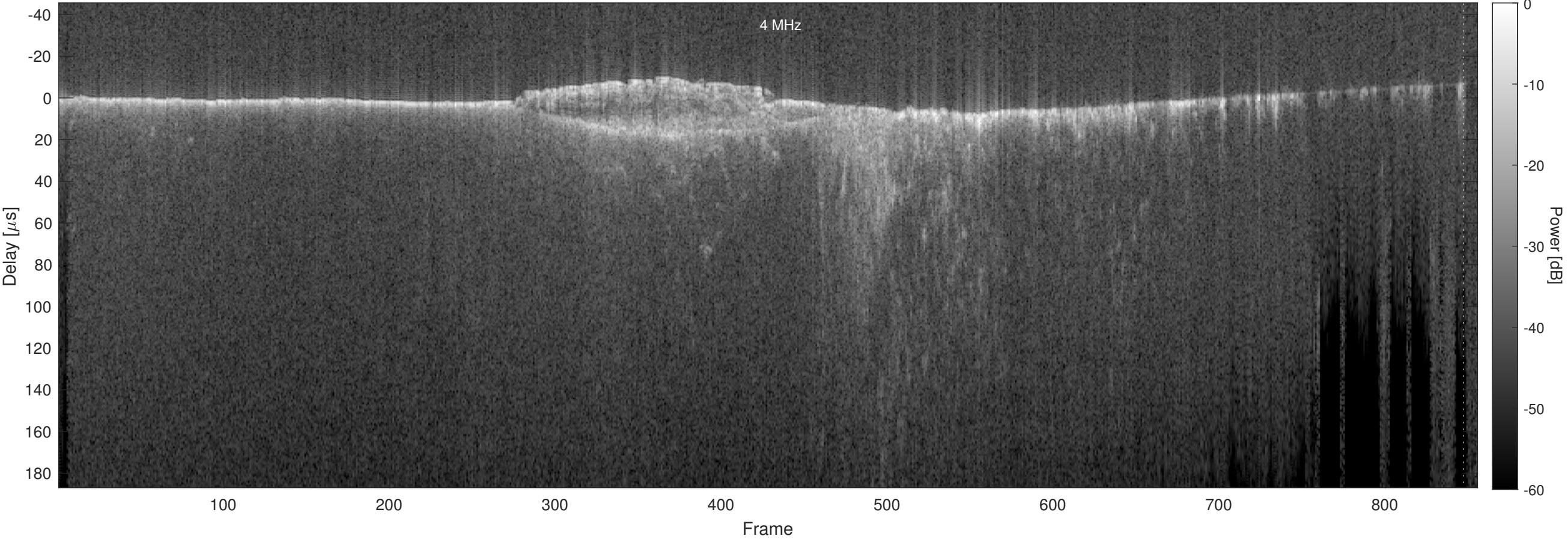
Orbit 9672, Optimized, No Window, Channel 2
