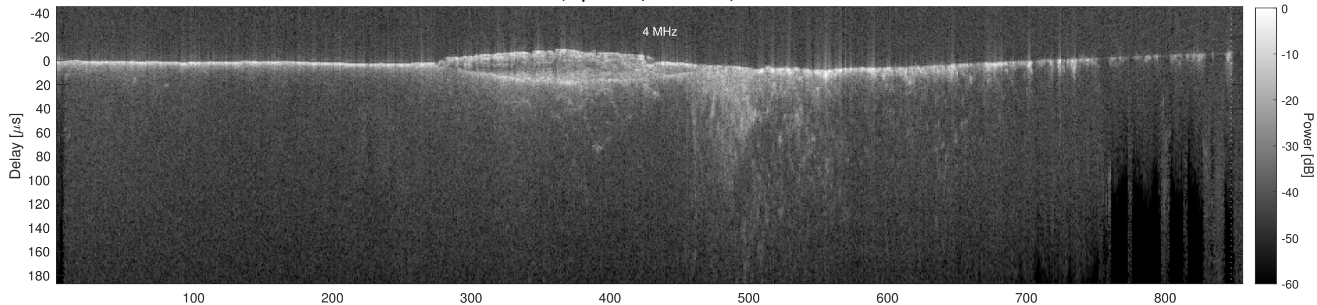
Orbit 9672, Cluttergram
