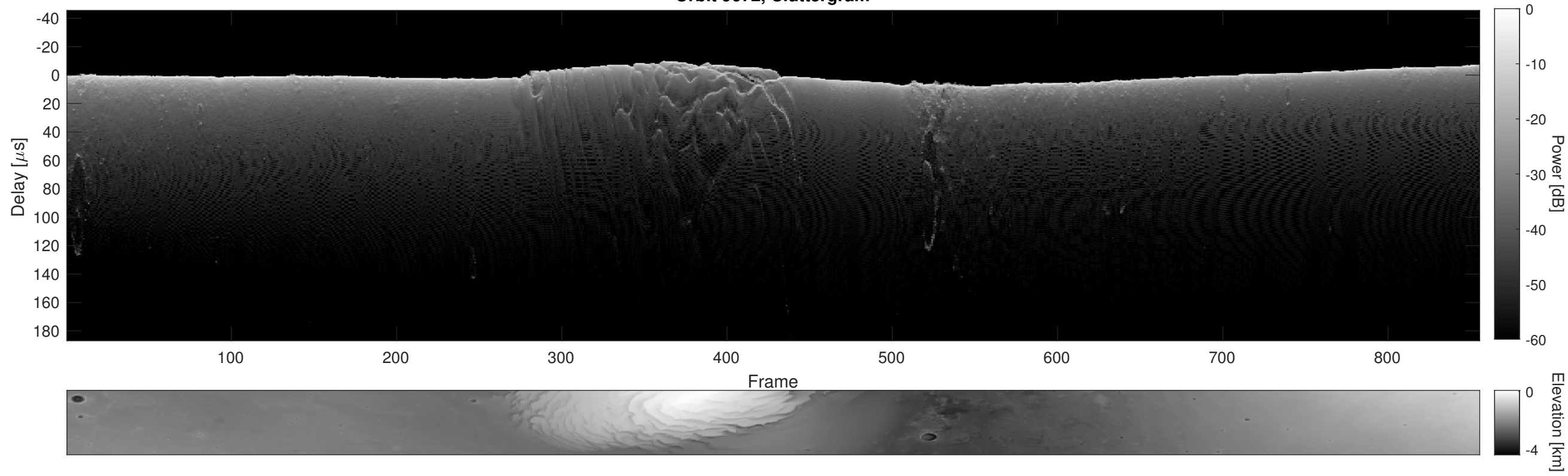
Orbit 9672, Cluttergram
