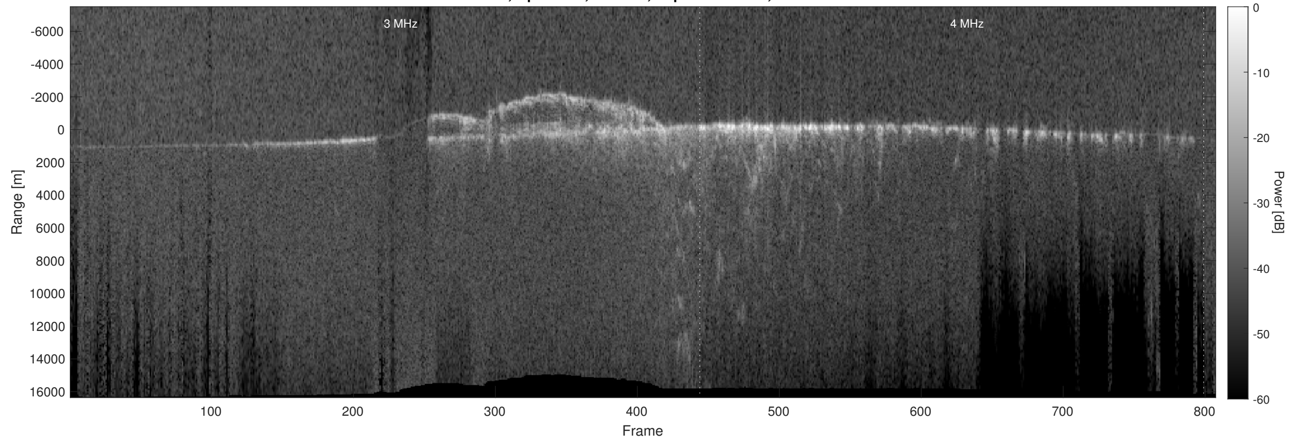
Orbit 9673, Optimized, Window, Depth-Corrected, Channel 2
