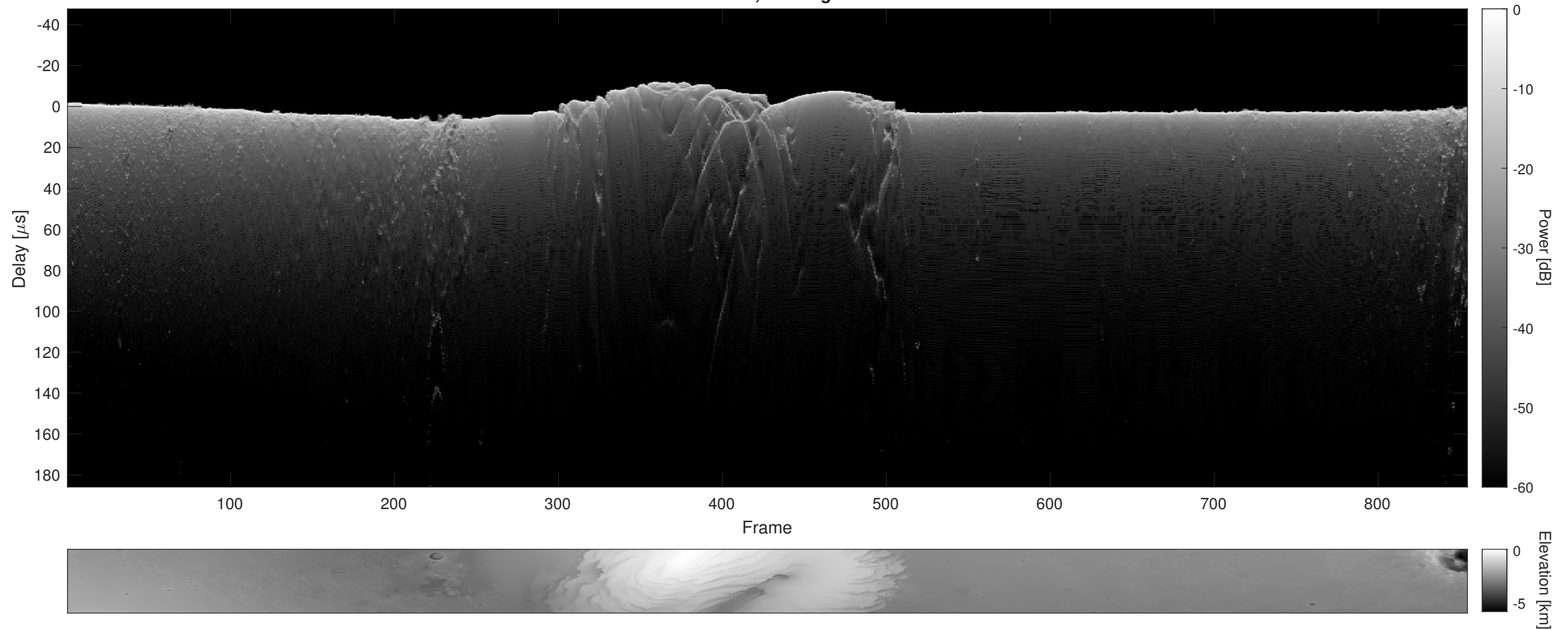
Orbit 9674, Cluttergram
