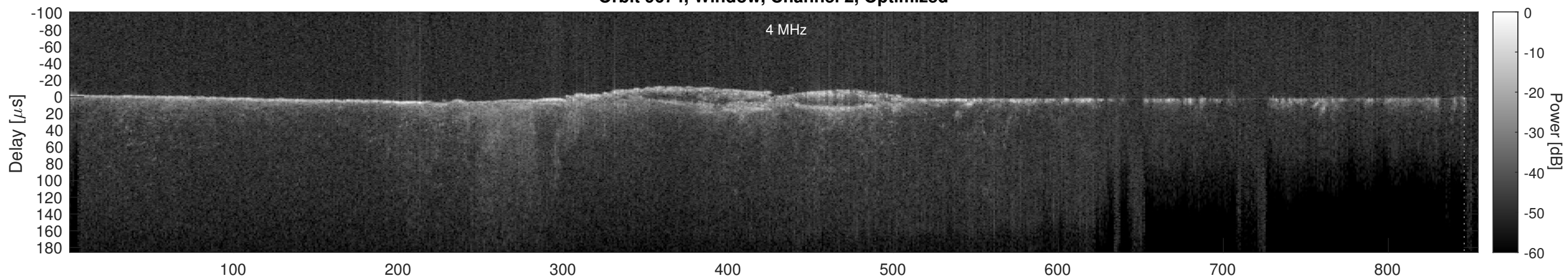
Orbit 9674, Cluttergram
