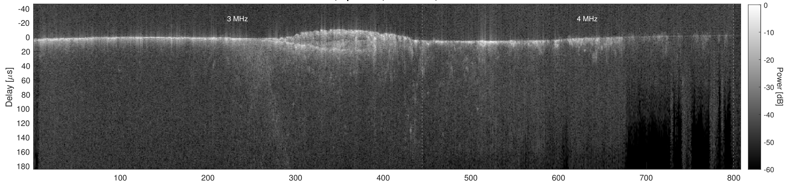
Orbit 9675, Cluttergram
