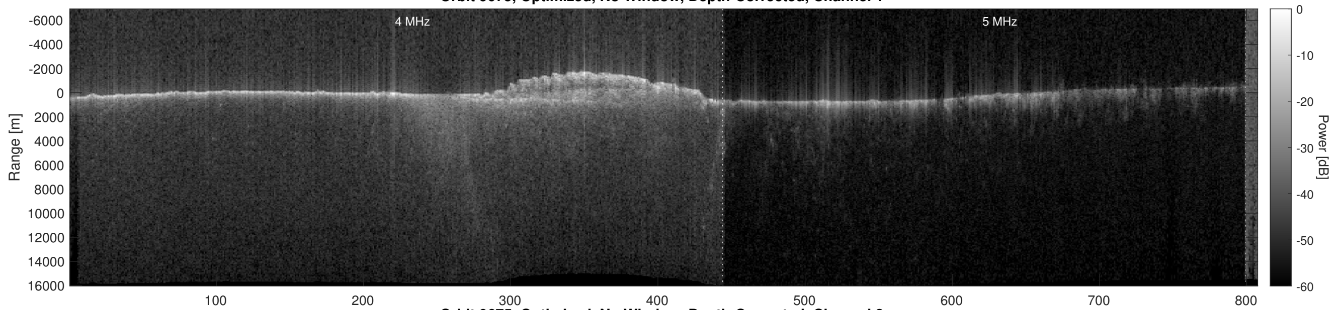
Orbit 9675, Optimized, No Window, Depth-Corrected, Channel 2
