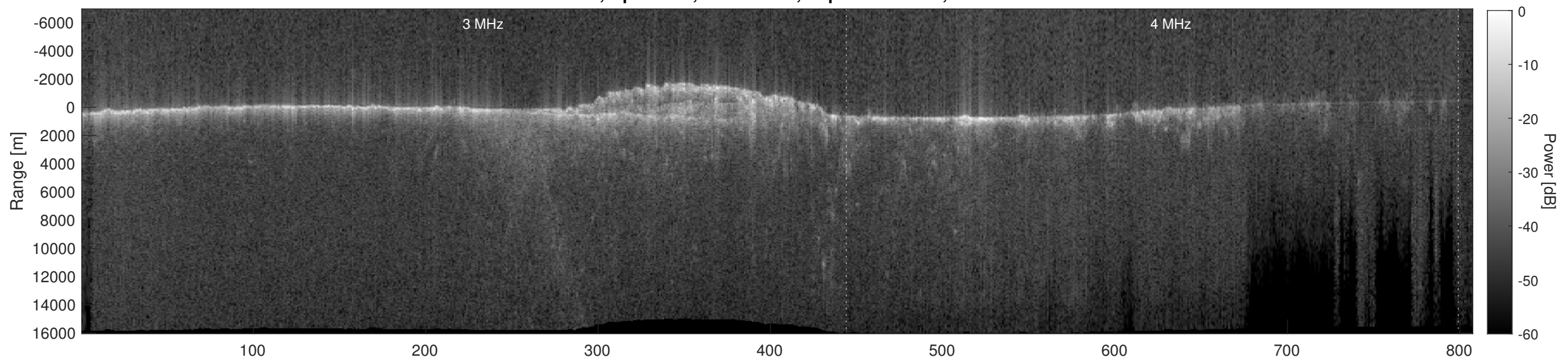
Orbit 9675, Depth-Corrected Cluttergram
