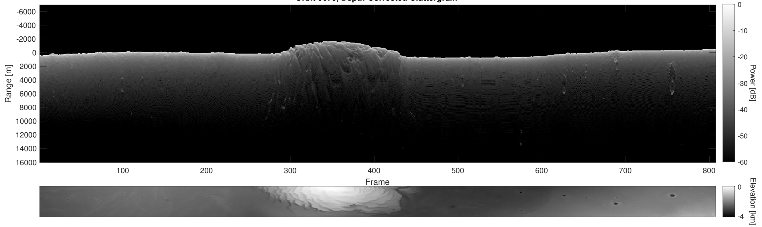
Orbit 9675, Depth-Corrected Cluttergram
