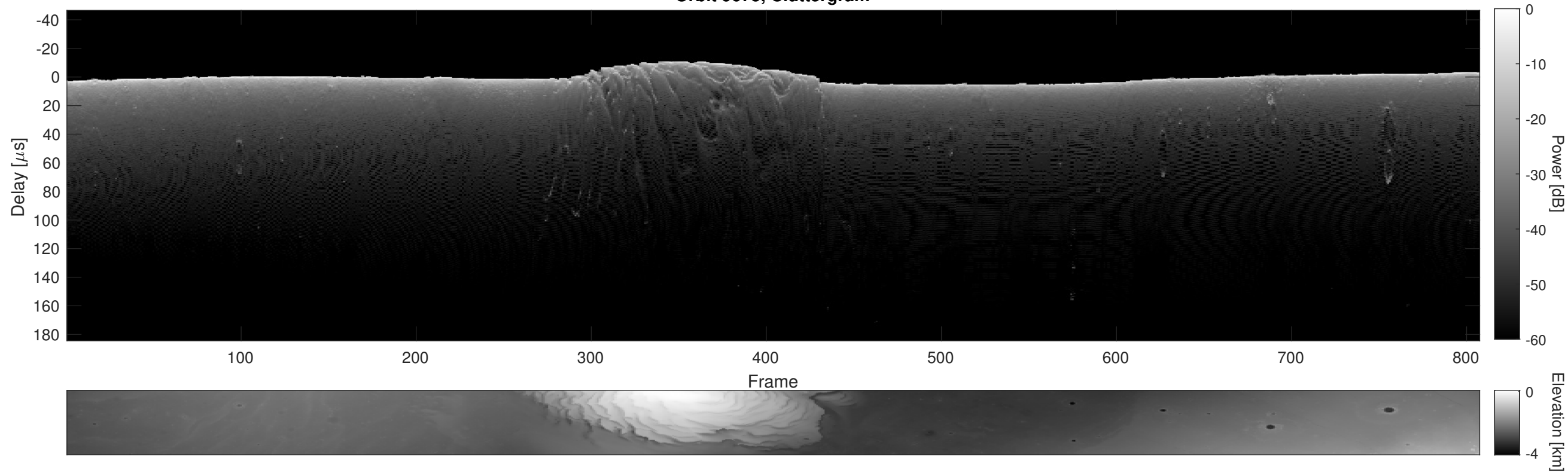
Orbit 9675, Cluttergram
