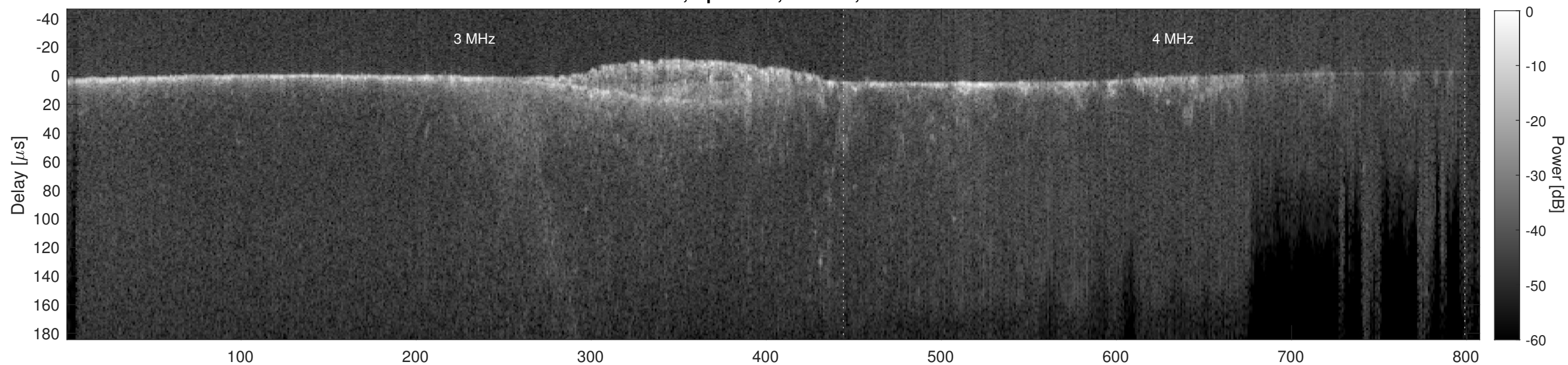
Orbit 9675, Cluttergram
