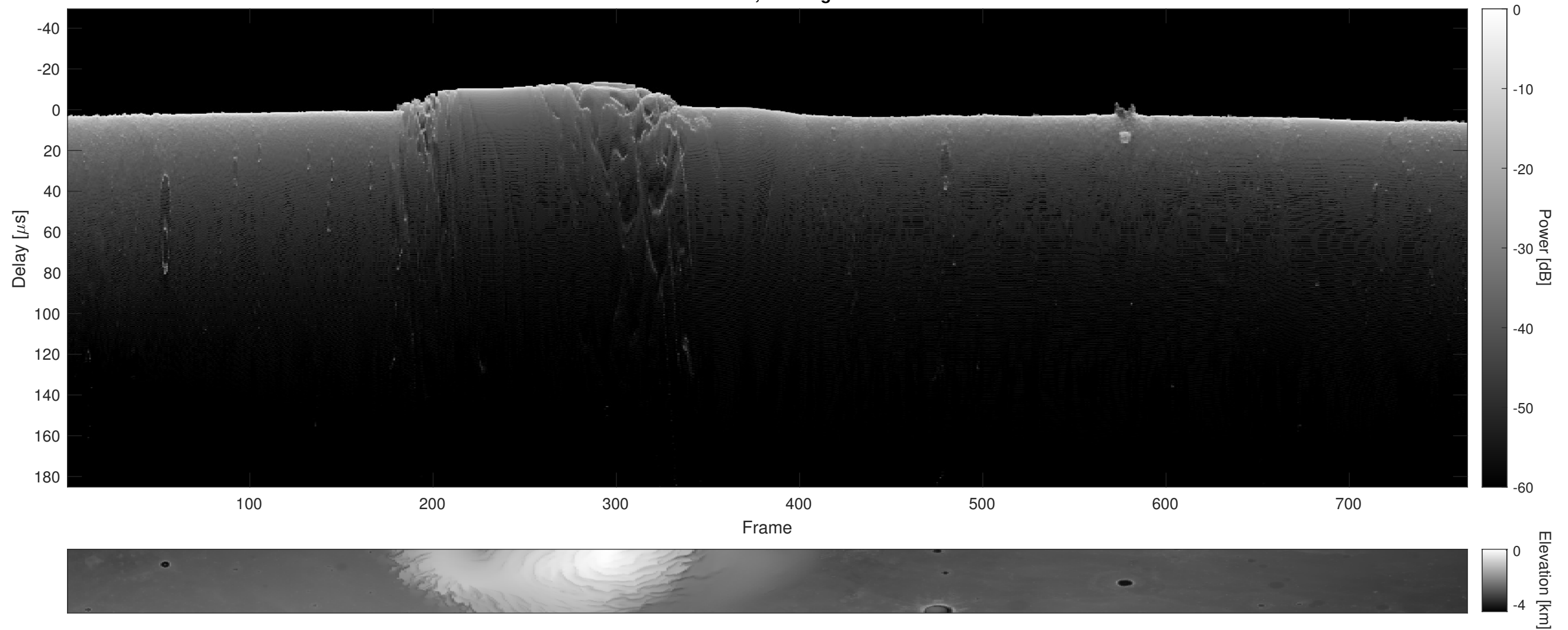
Orbit 9676, Cluttergram
