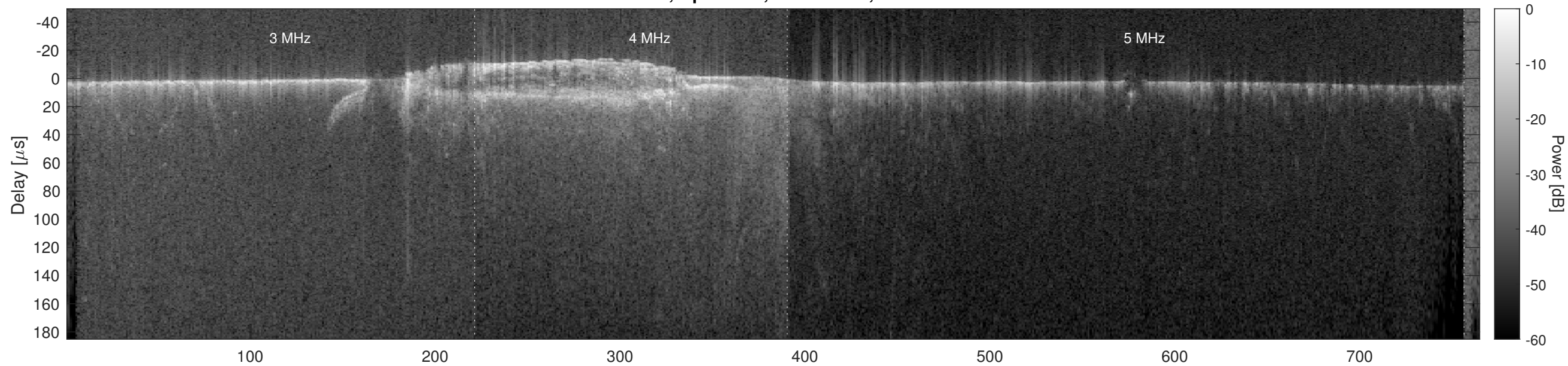
Orbit 9676, Optimized, No Window, Channel 2
