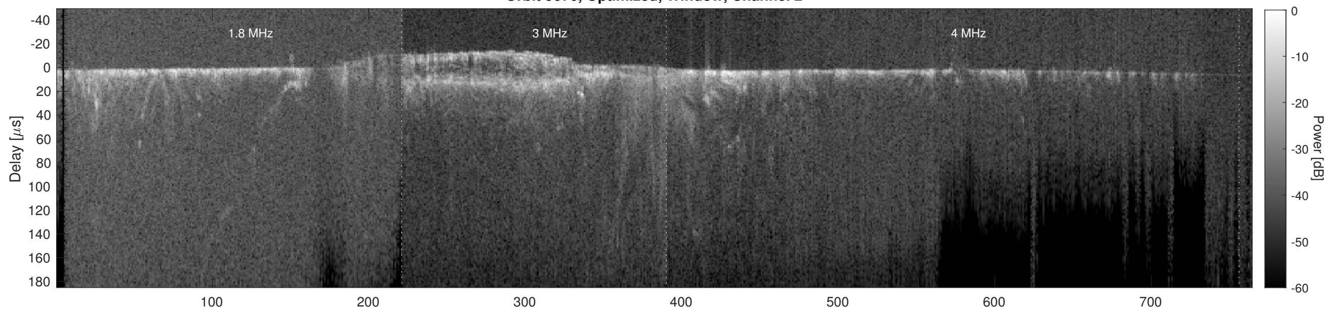
Orbit 9676, Cluttergram
