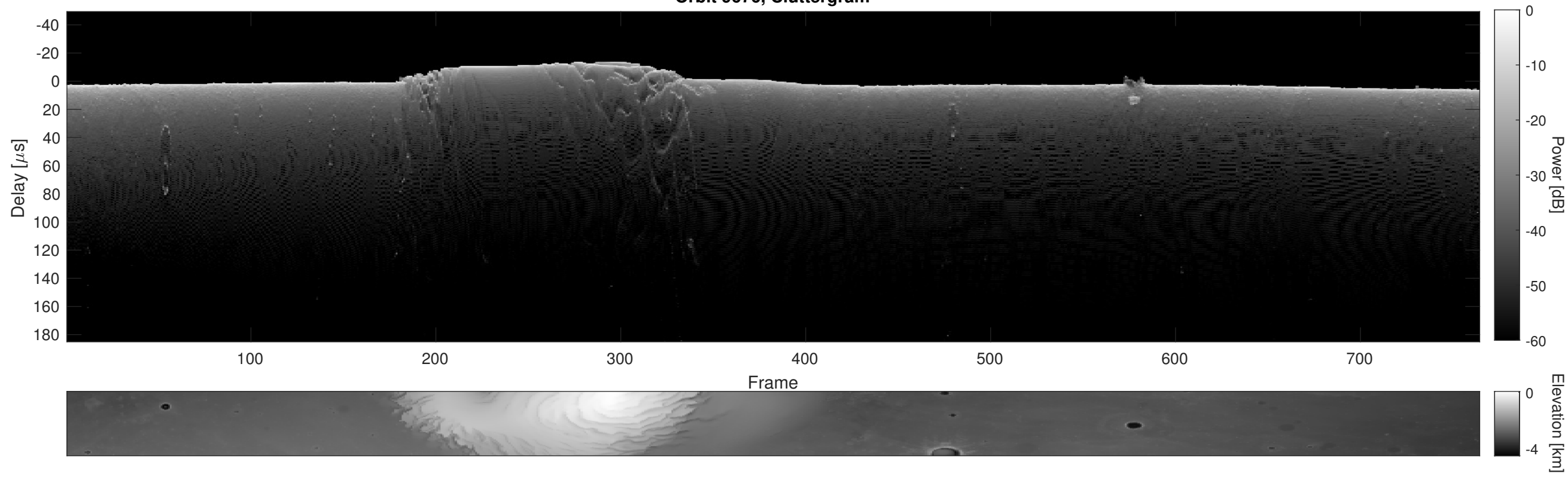
Orbit 9676, Cluttergram
