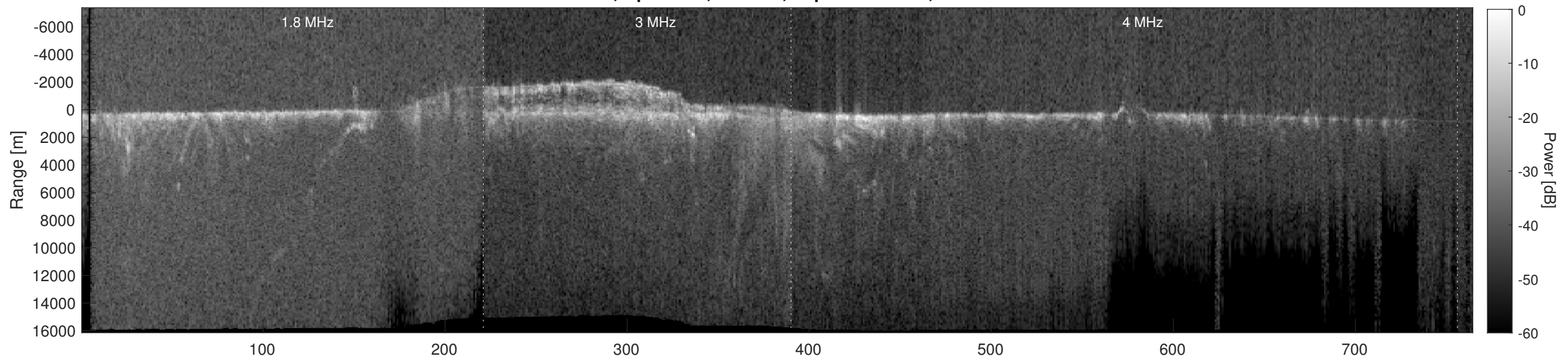
Orbit 9676, Depth-Corrected Cluttergram
