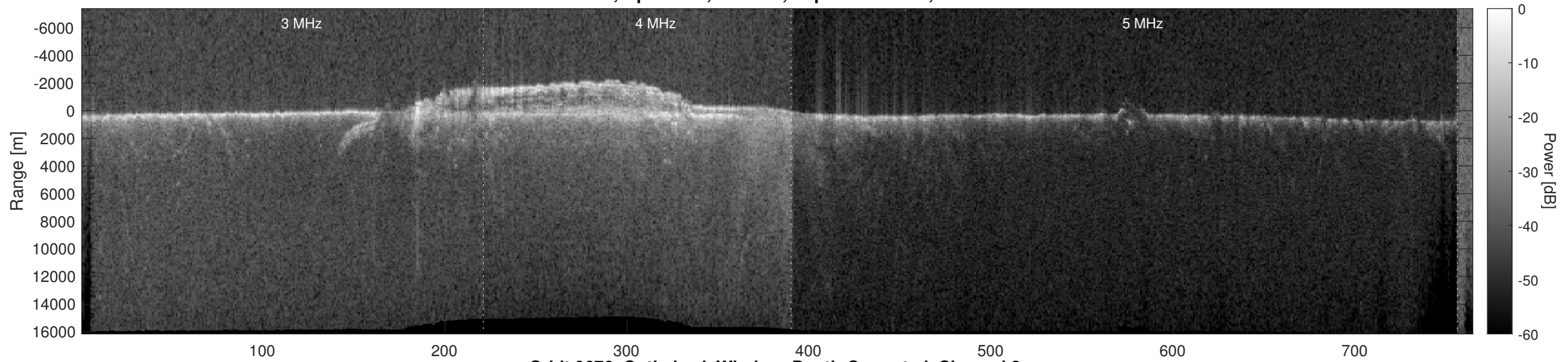
Orbit 9676, Optimized, Window, Depth-Corrected, Channel 2
