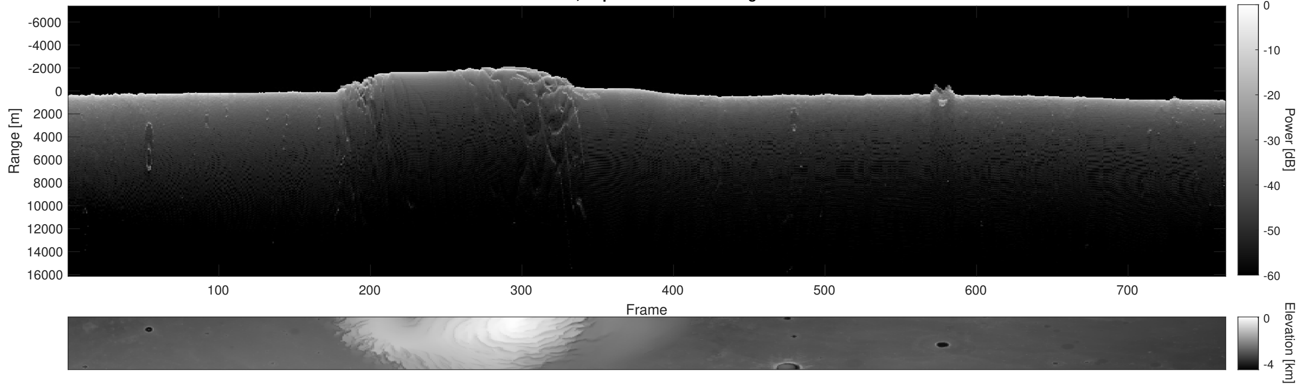
Orbit 9676, Depth-Corrected Cluttergram
