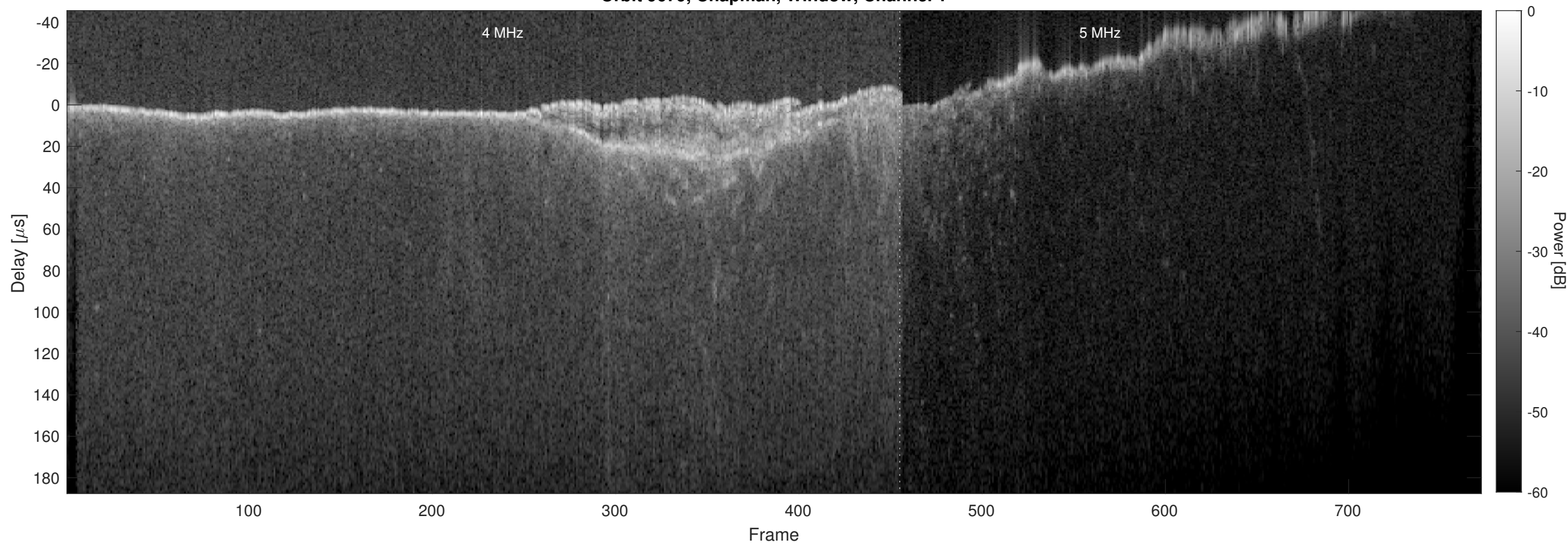
Orbit 9679, Chapman, Window, Channel 2
