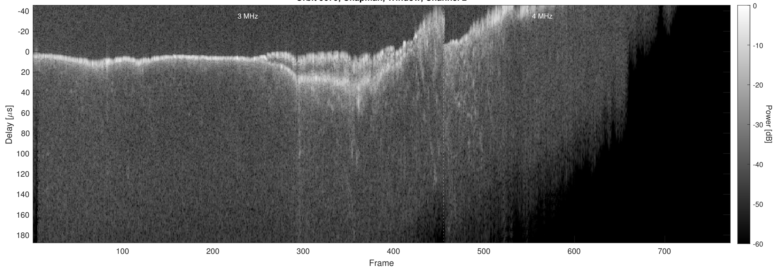
Orbit 9679, Chapman, Window, Channel 2
