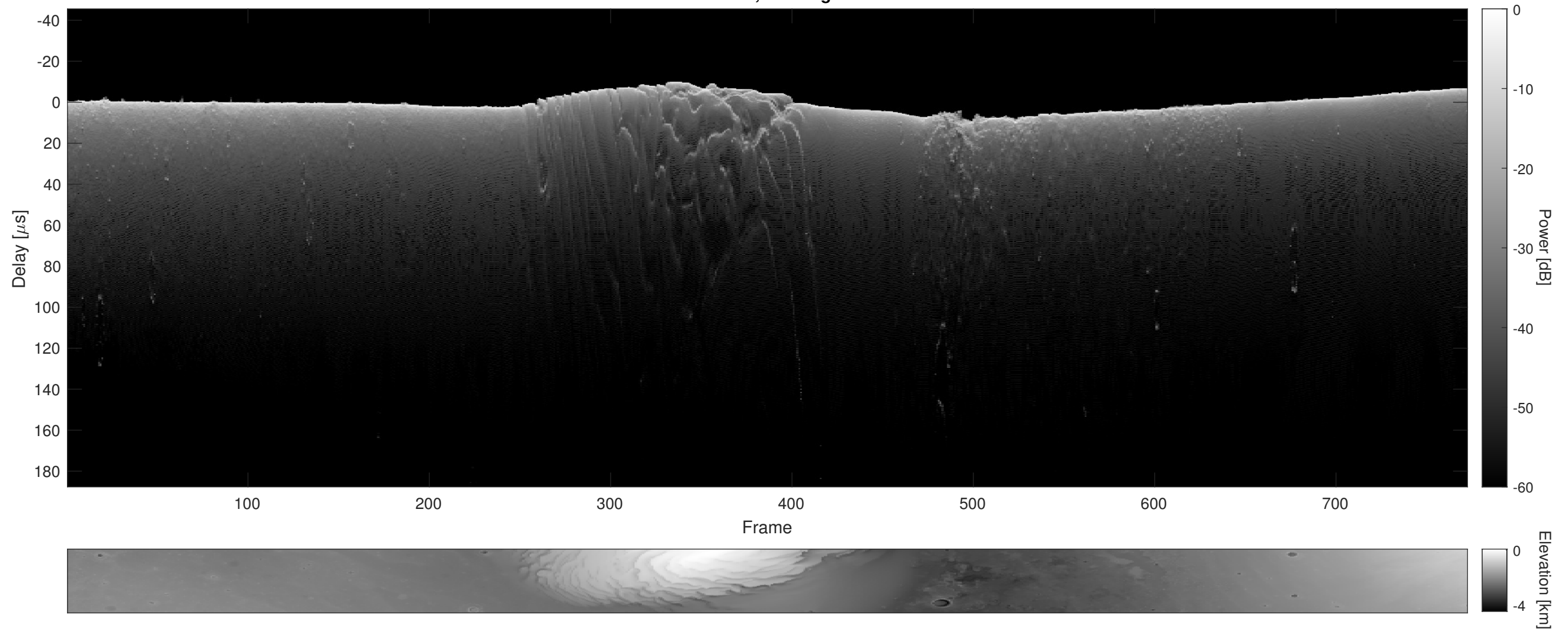
Orbit 9679, Cluttergram
