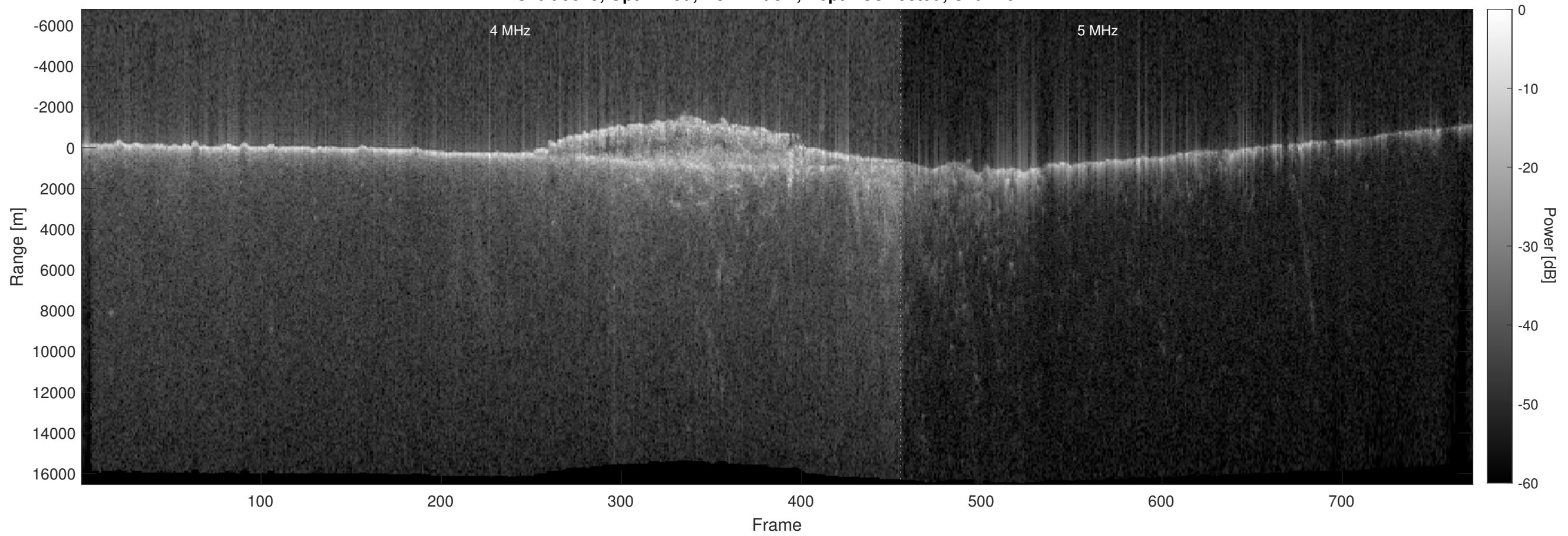
Orbit 9679, Optimized, No Window, Depth-Corrected, Channel 2
