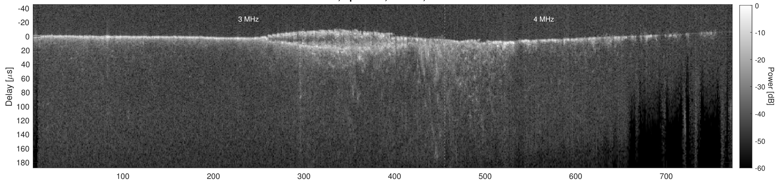
Orbit 9679, Cluttergram
