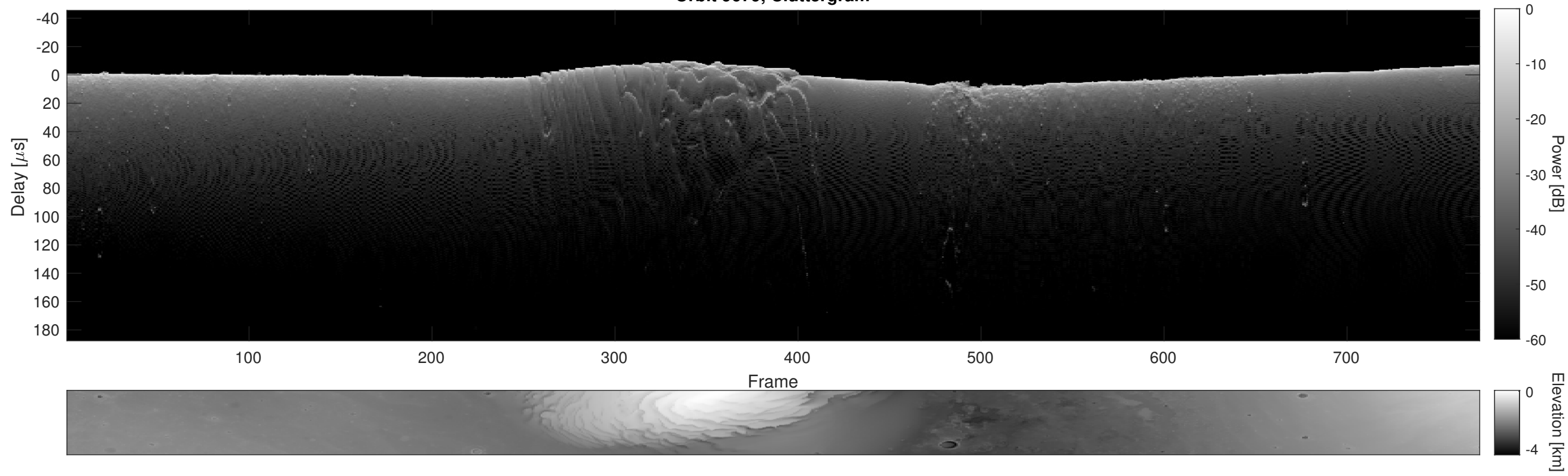
Orbit 9679, Cluttergram
