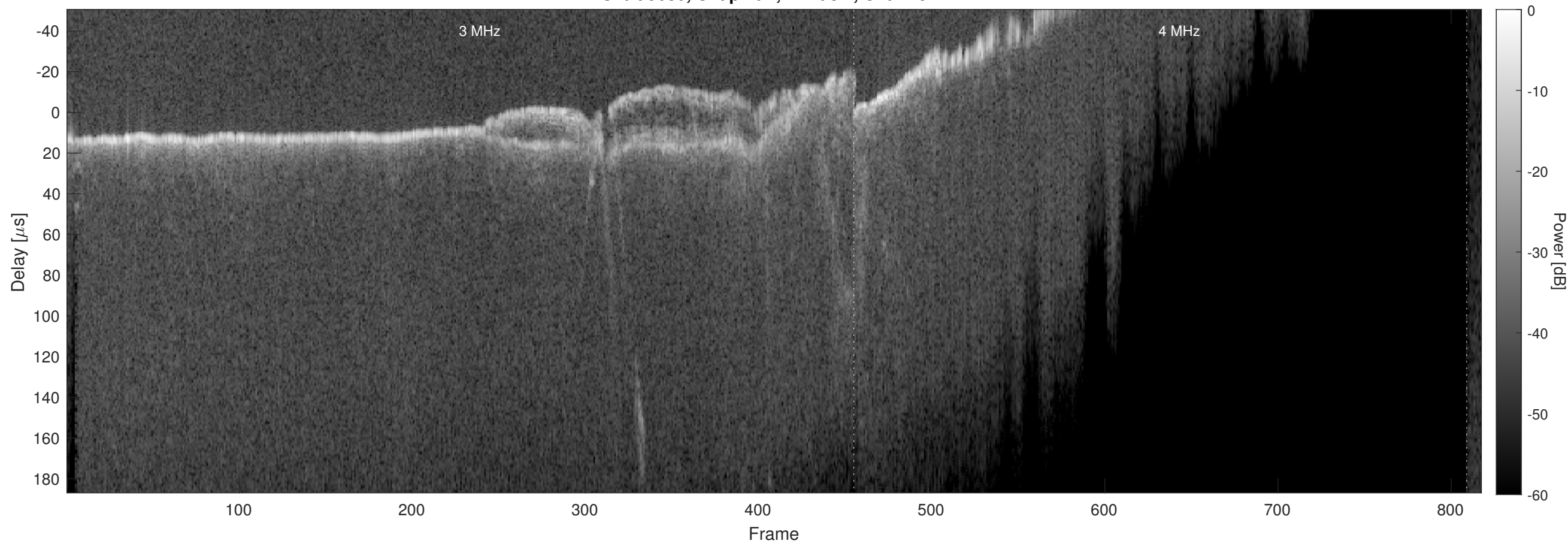
Orbit 9680, Chapman, Window, Channel 2
