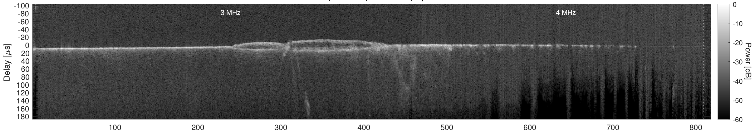
Orbit 9680, Cluttergram
