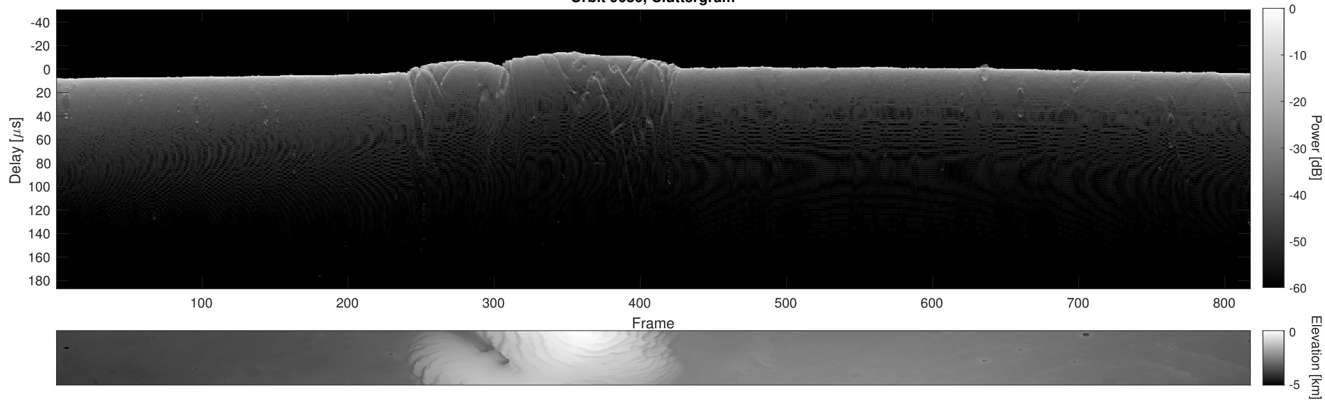
Orbit 9680, Cluttergram
