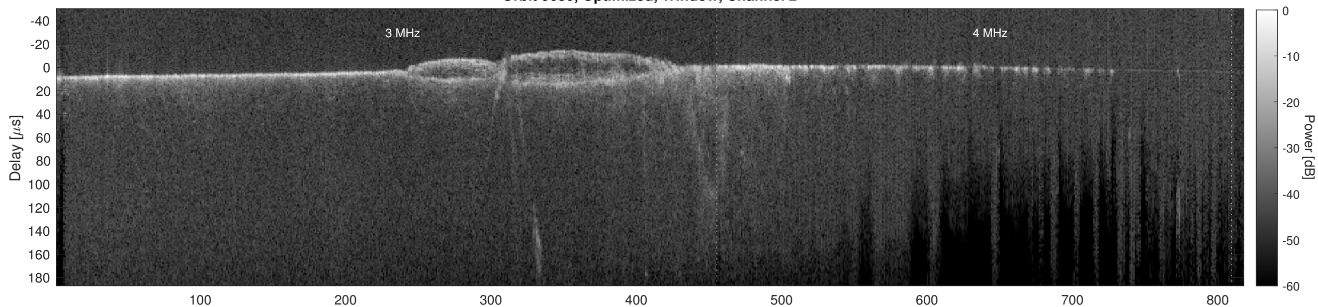
Orbit 9680, Cluttergram
