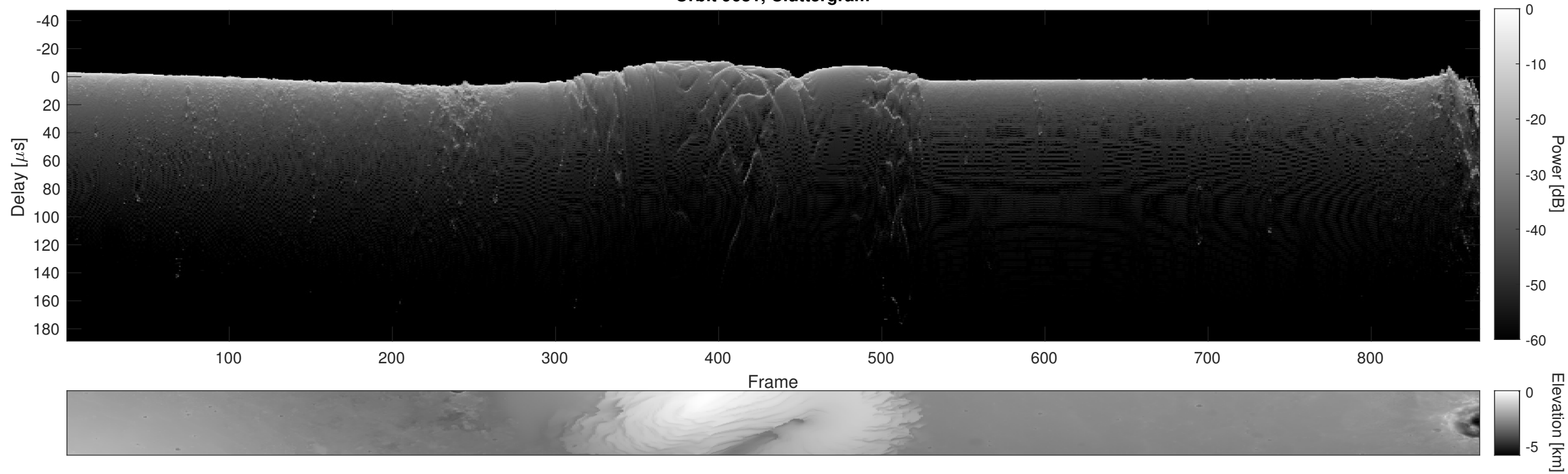
Orbit 9681, Cluttergram
