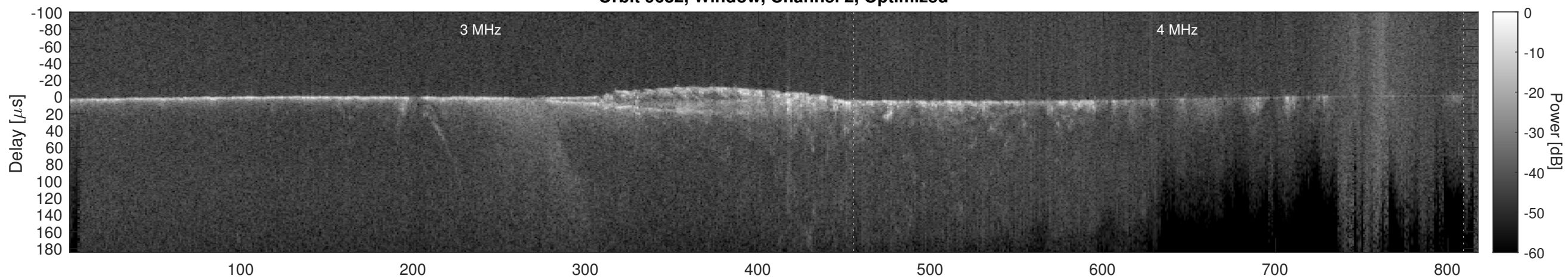
Orbit 9682, Cluttergram
