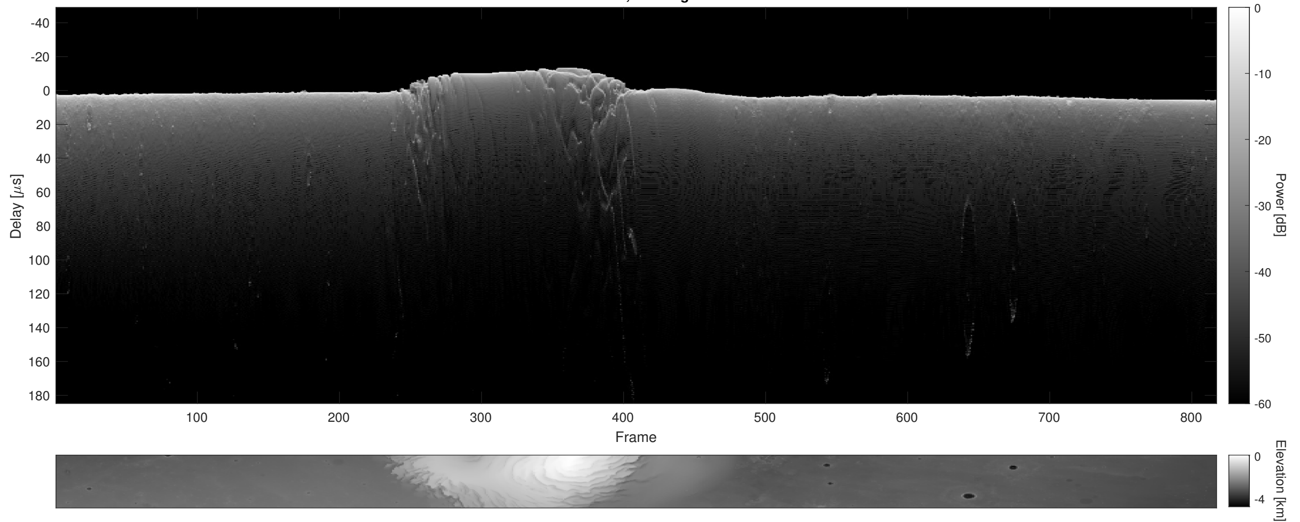
Orbit 9683, Cluttergram
