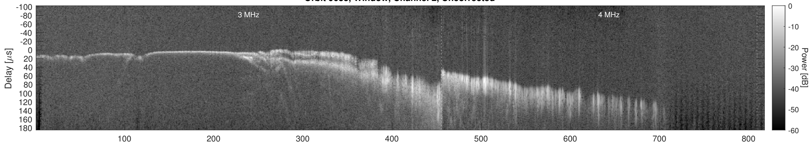
Orbit 9683, Window, Channel 2, Chapman
