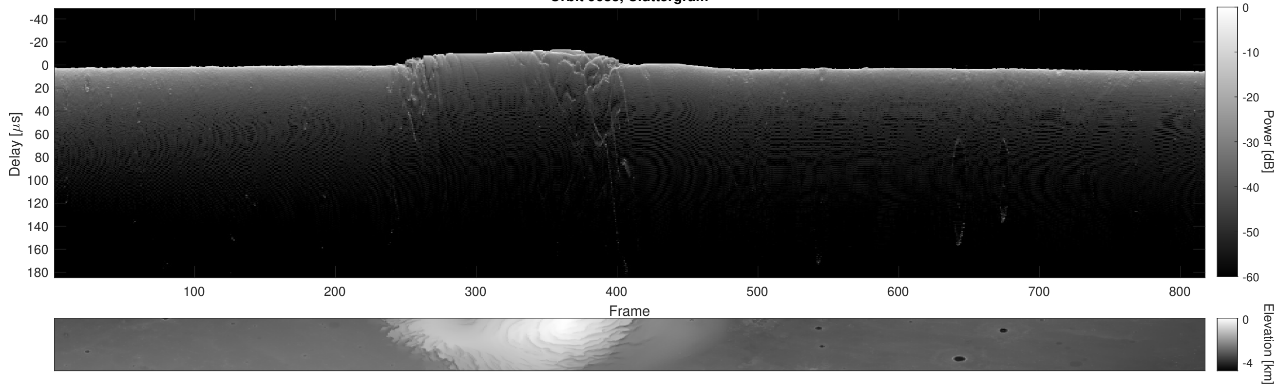
Orbit 9683, Cluttergram
