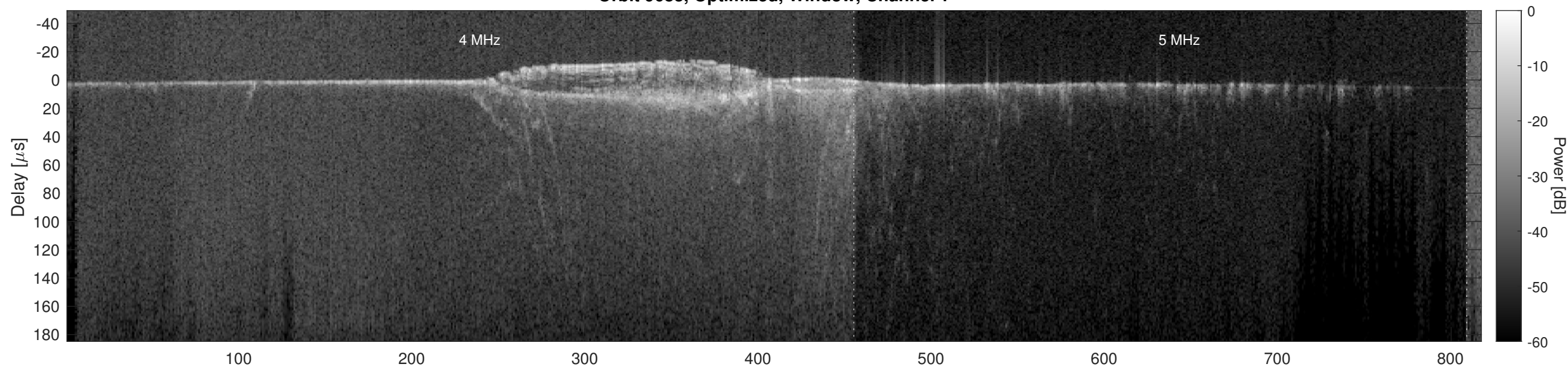
Orbit 9683, Optimized, Window, Channel 2
