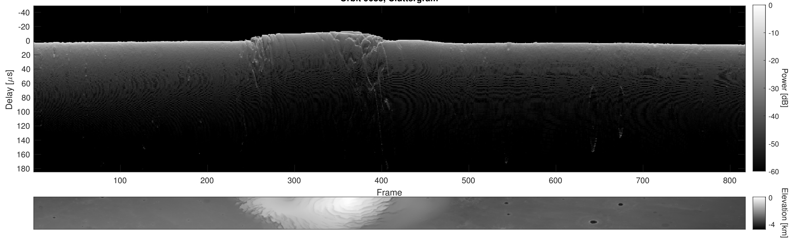
Orbit 9683, Cluttergram
