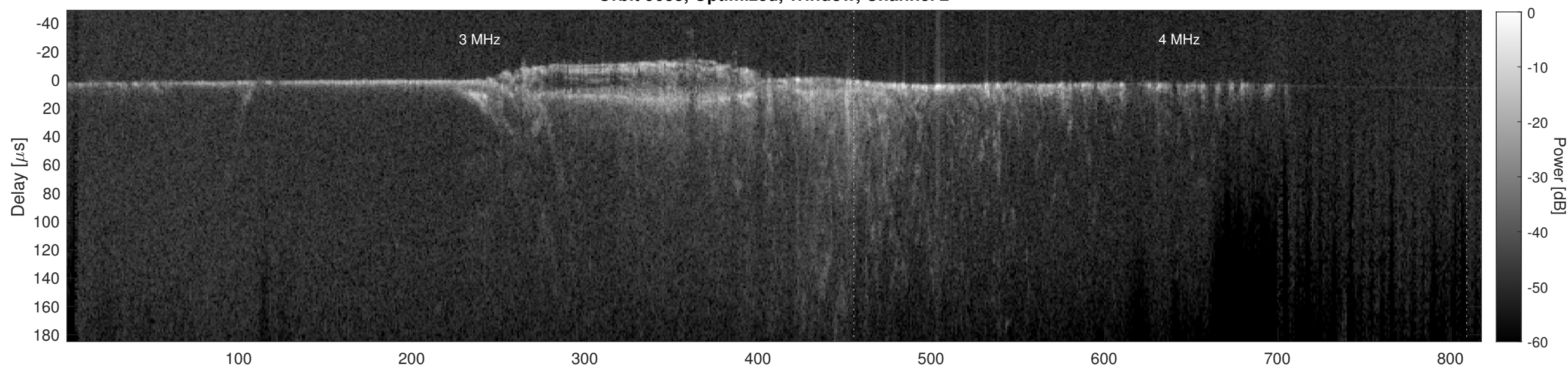
Orbit 9683, Cluttergram
