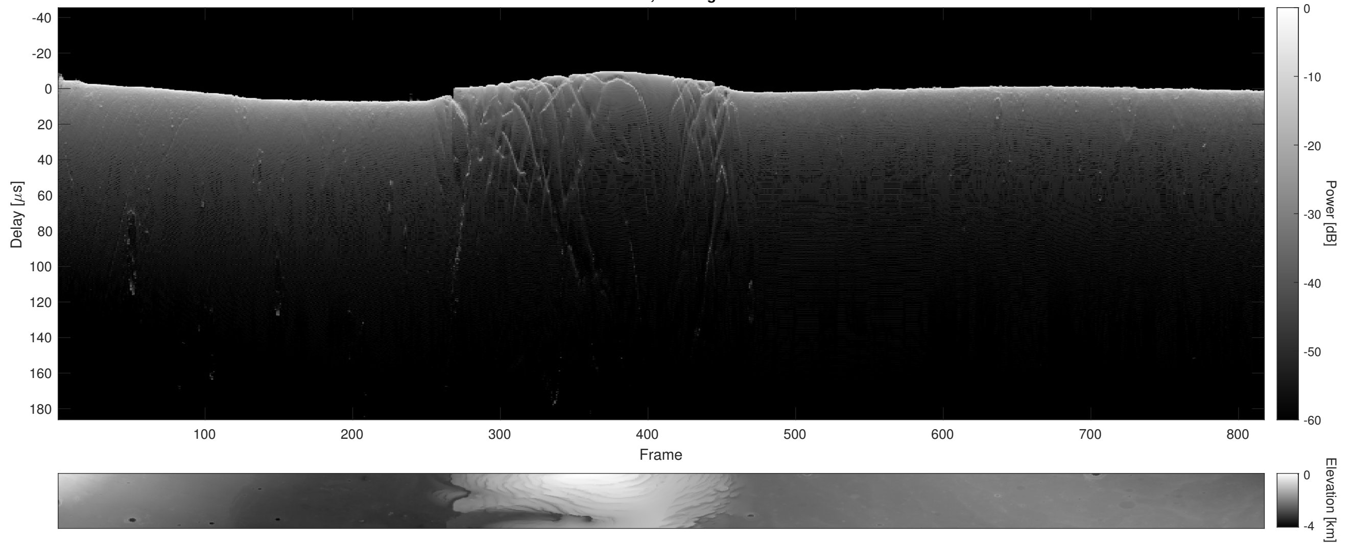
Orbit 9684, Cluttergram
