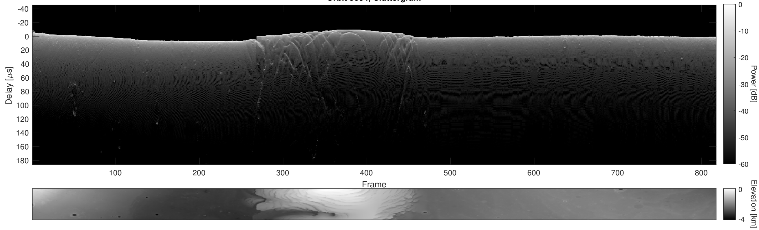
Orbit 9684, Cluttergram
