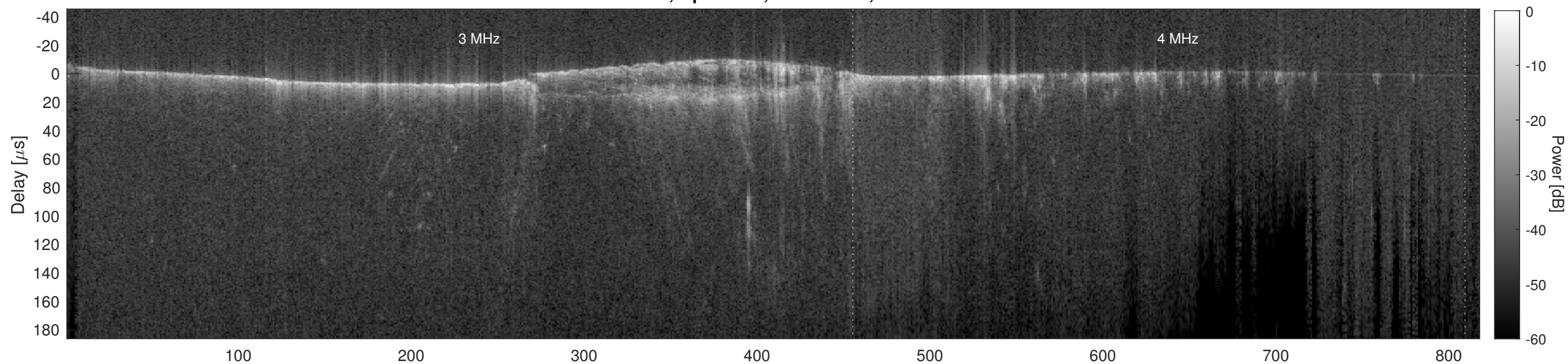
Orbit 9684, Cluttergram
