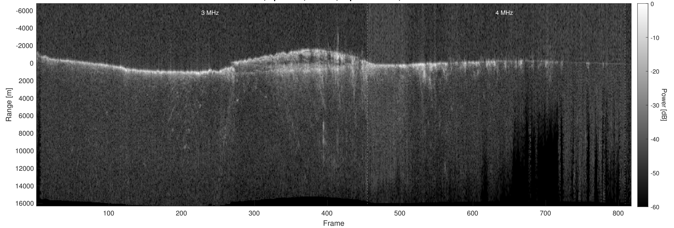
Orbit 9684, Optimized, Window, Depth-Corrected, Channel 2
