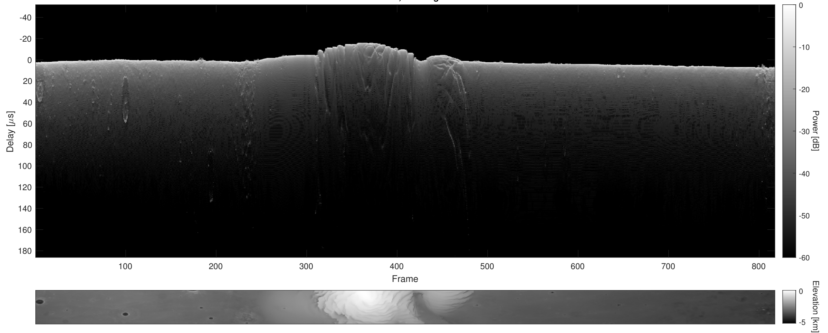
Orbit 9685, Cluttergram
