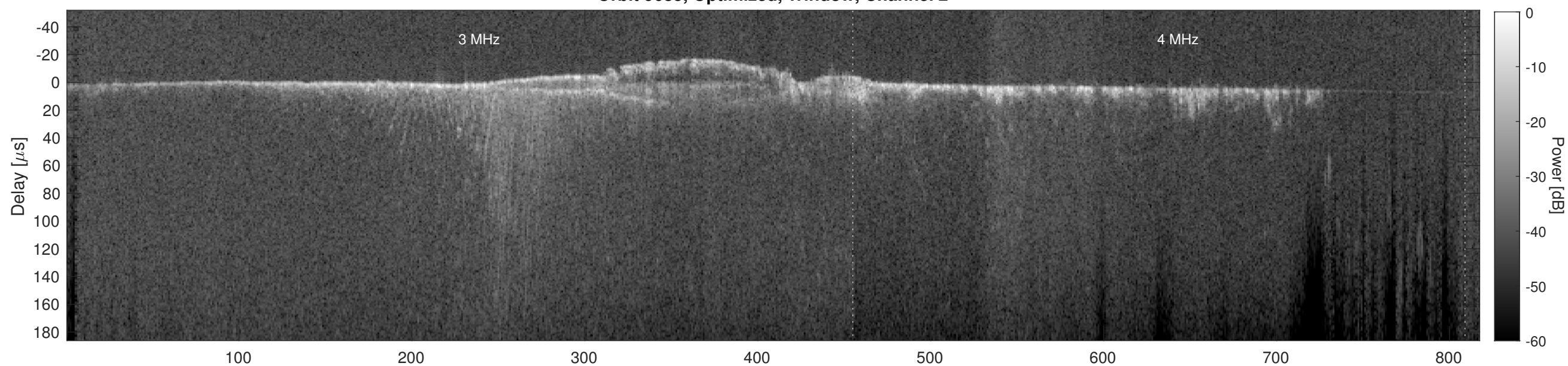
Orbit 9685, Cluttergram
