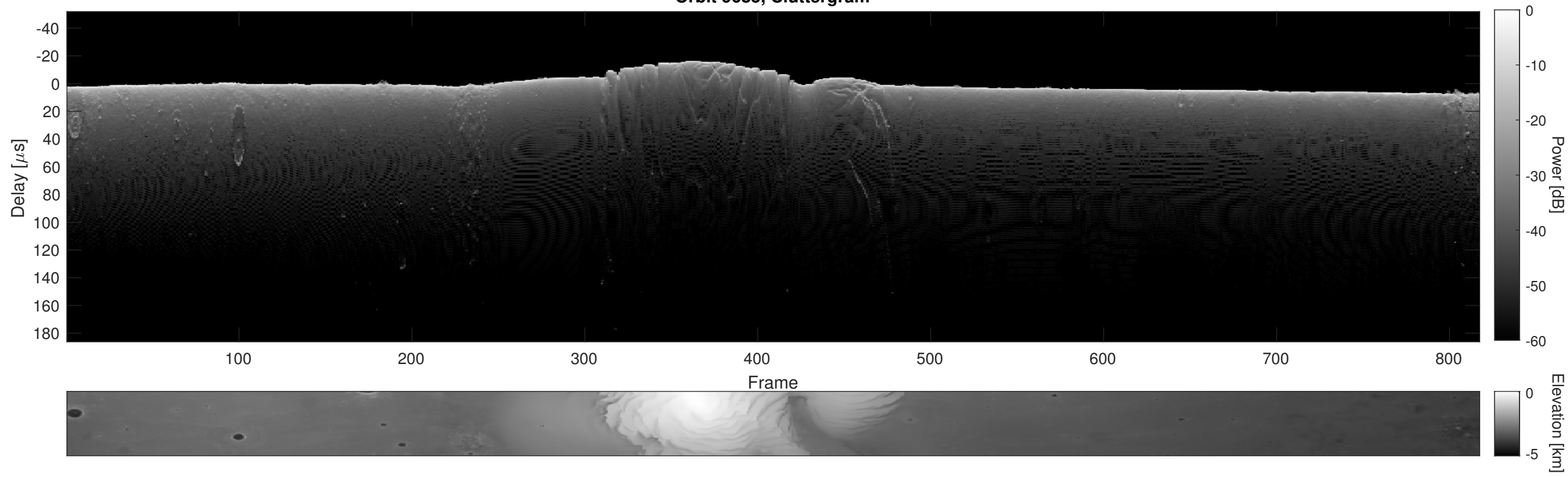
Orbit 9685, Cluttergram
