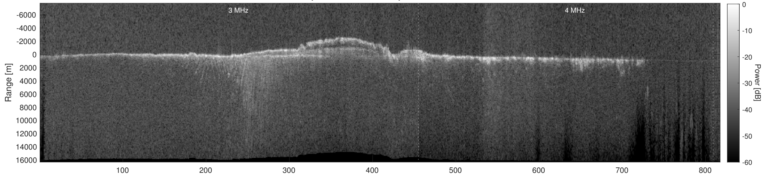
Orbit 9685, Depth-Corrected Cluttergram
