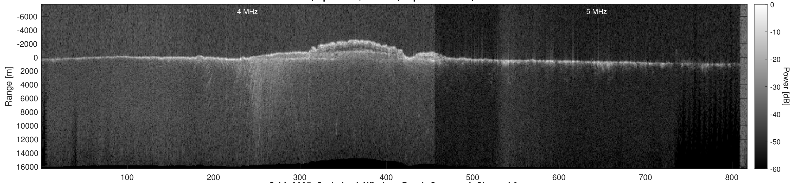
Orbit 9685, Optimized, Window, Depth-Corrected, Channel 2
