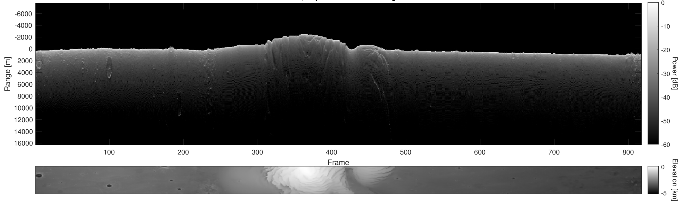
Orbit 9685, Depth-Corrected Cluttergram
