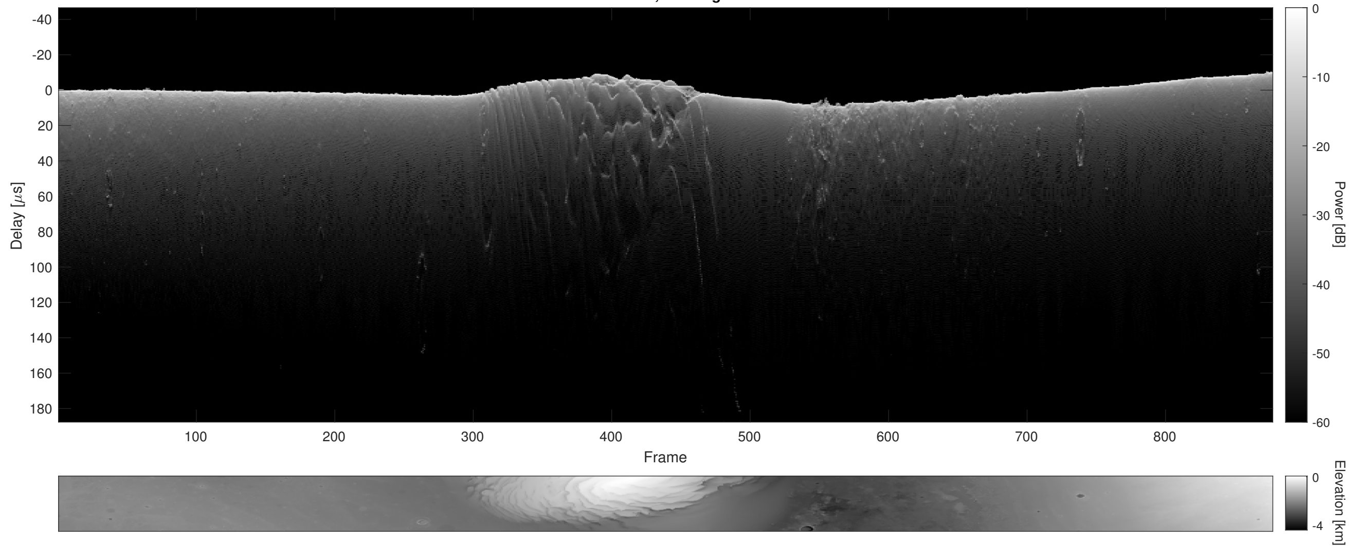
Orbit 9686, Cluttergram
