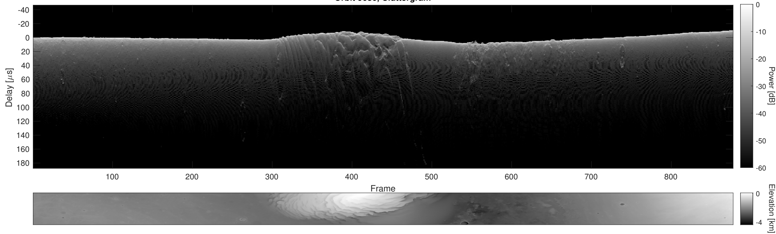
Orbit 9686, Cluttergram
