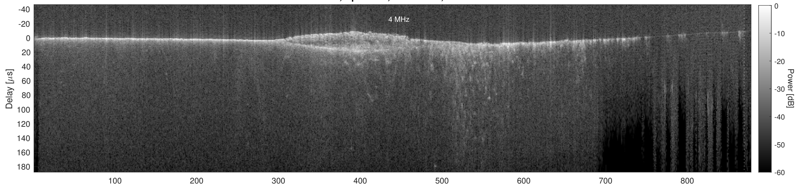
Orbit 9686, Cluttergram
