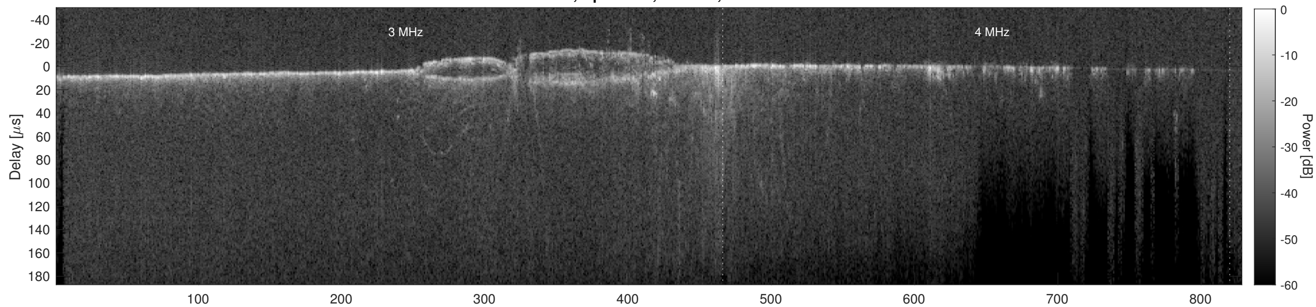
Orbit 9687, Cluttergram
