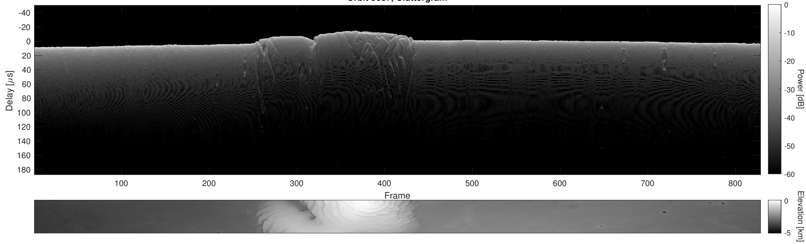
Orbit 9687, Cluttergram
