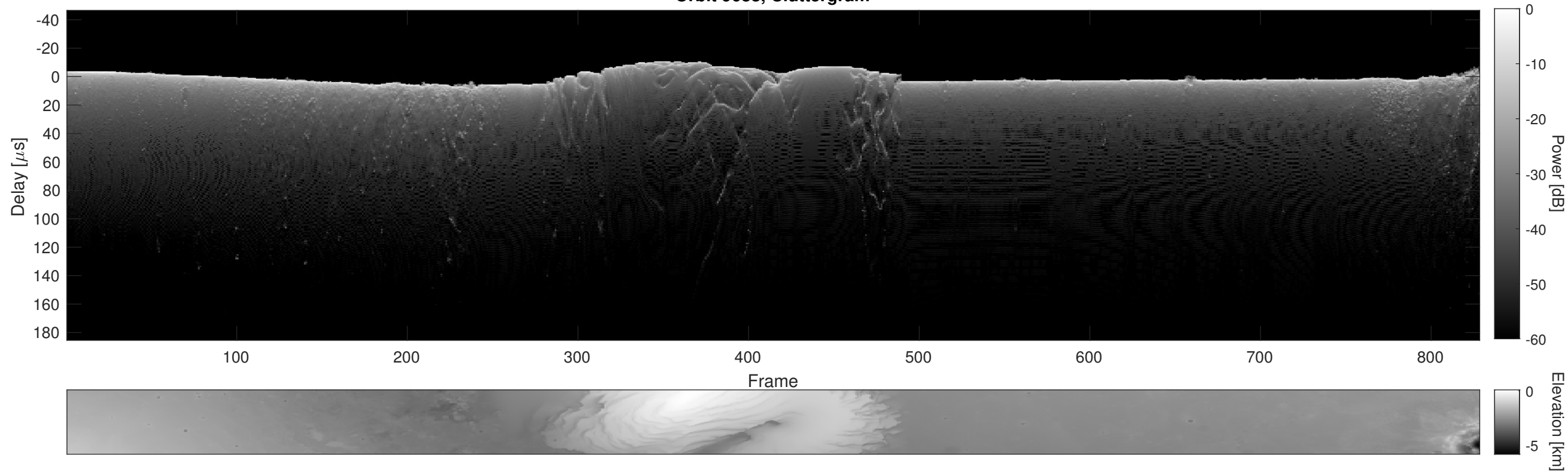
Orbit 9688, Cluttergram
