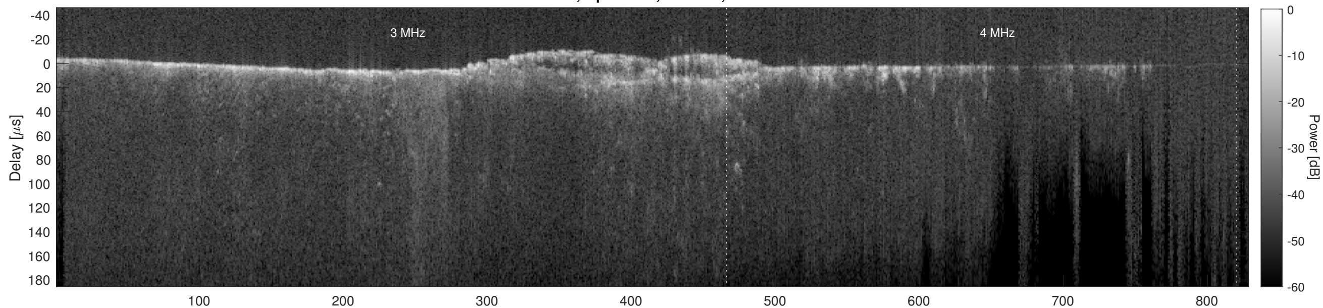
Orbit 9688, Cluttergram
