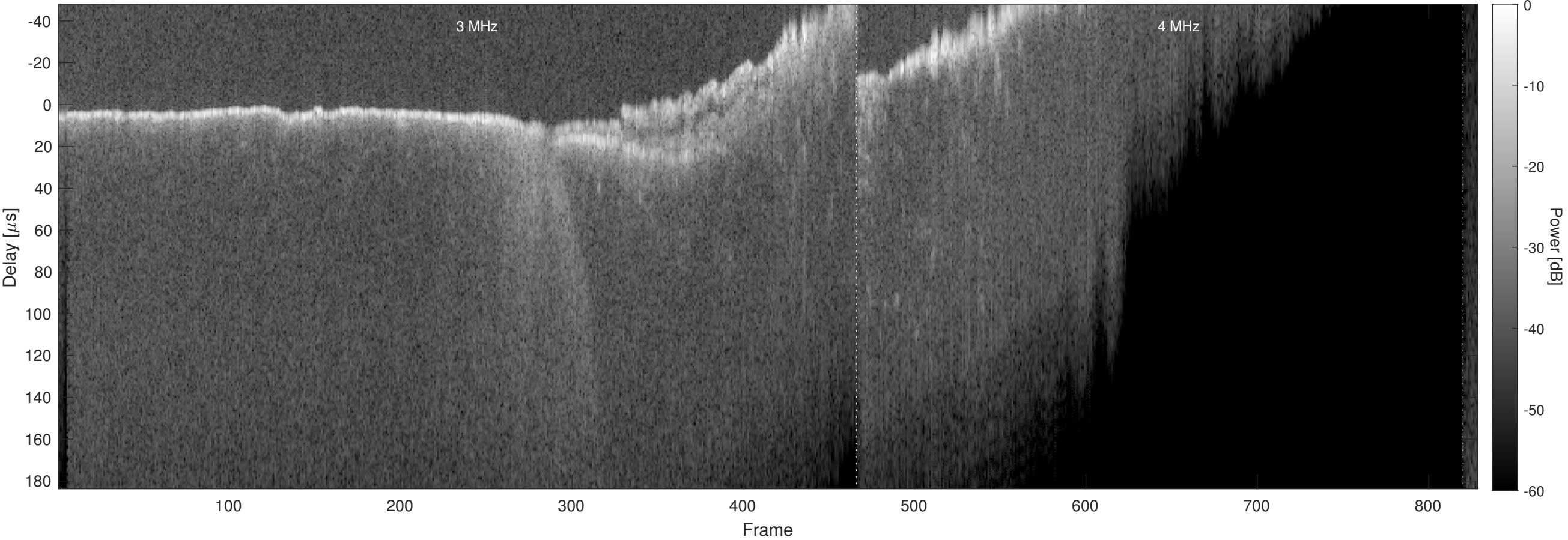
Orbit 9689, Chapman, Window, Channel 2
