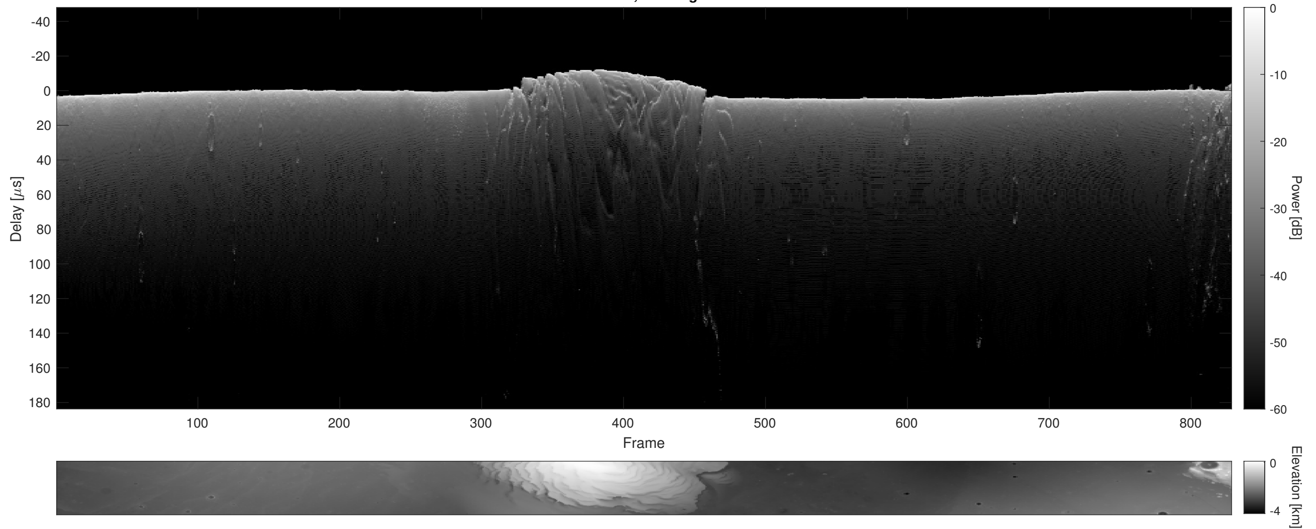
Orbit 9689, Cluttergram
