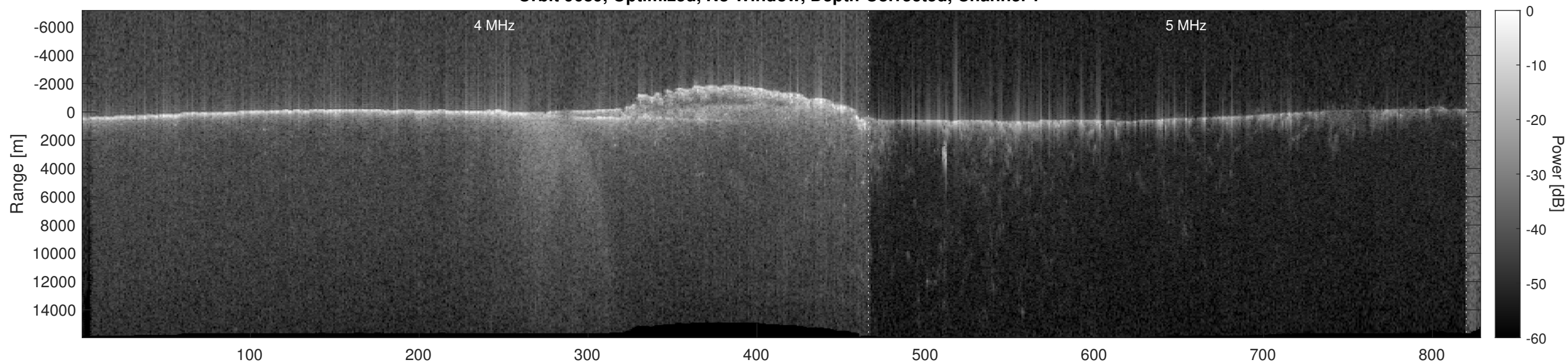
Orbit 9689, Optimized, No Window, Depth-Corrected, Channel 2
