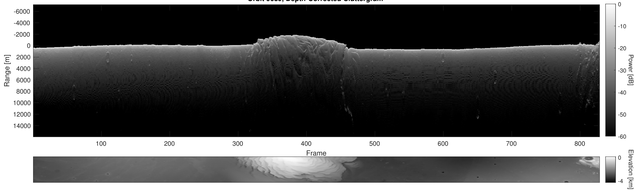
Orbit 9689, Depth-Corrected Cluttergram
