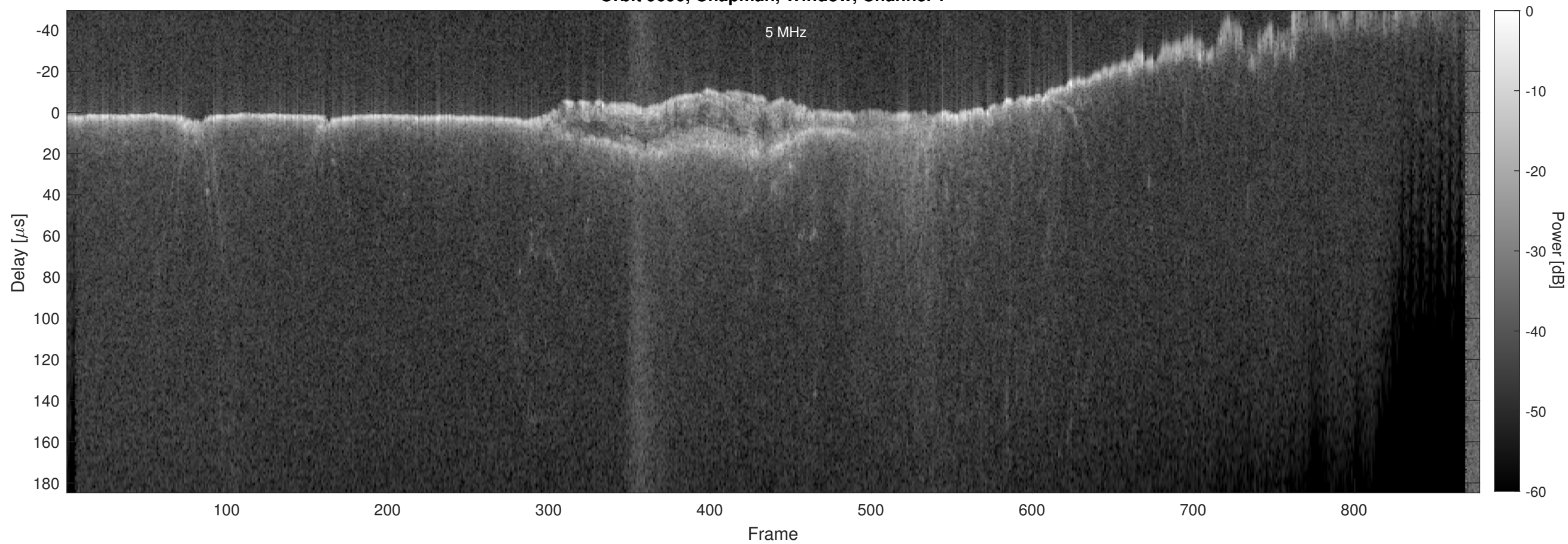
Orbit 9690, Chapman, Window, Channel 2
