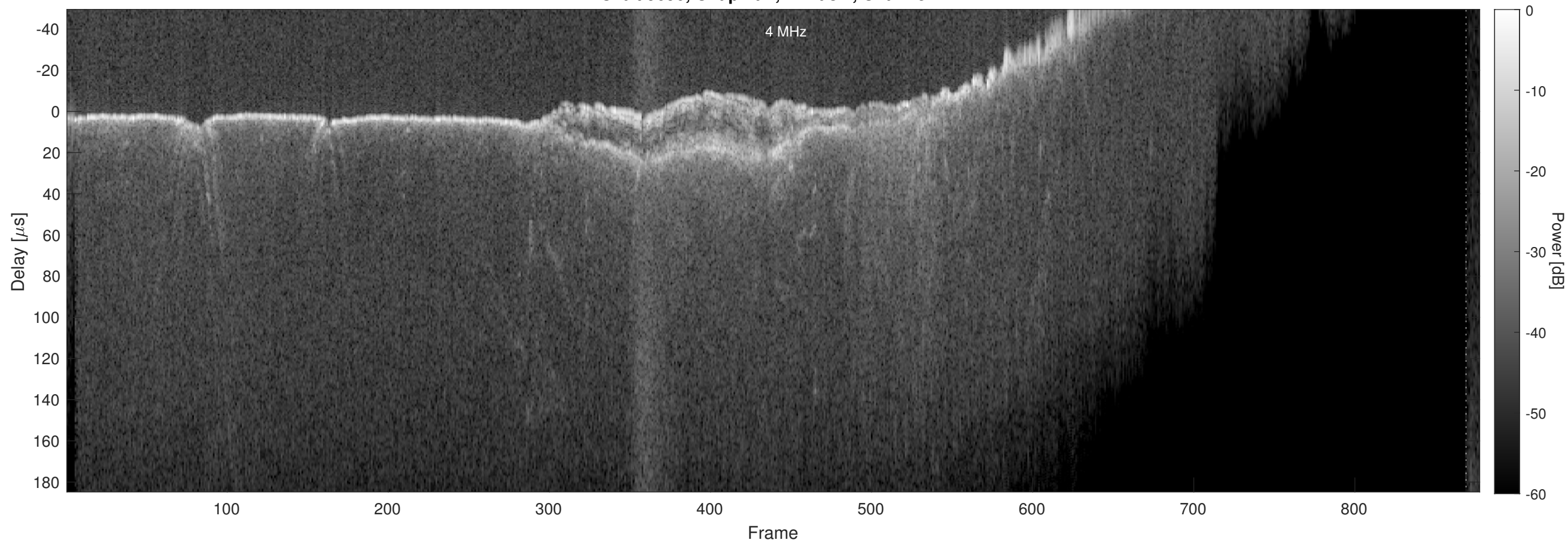
Orbit 9690, Chapman, Window, Channel 2
