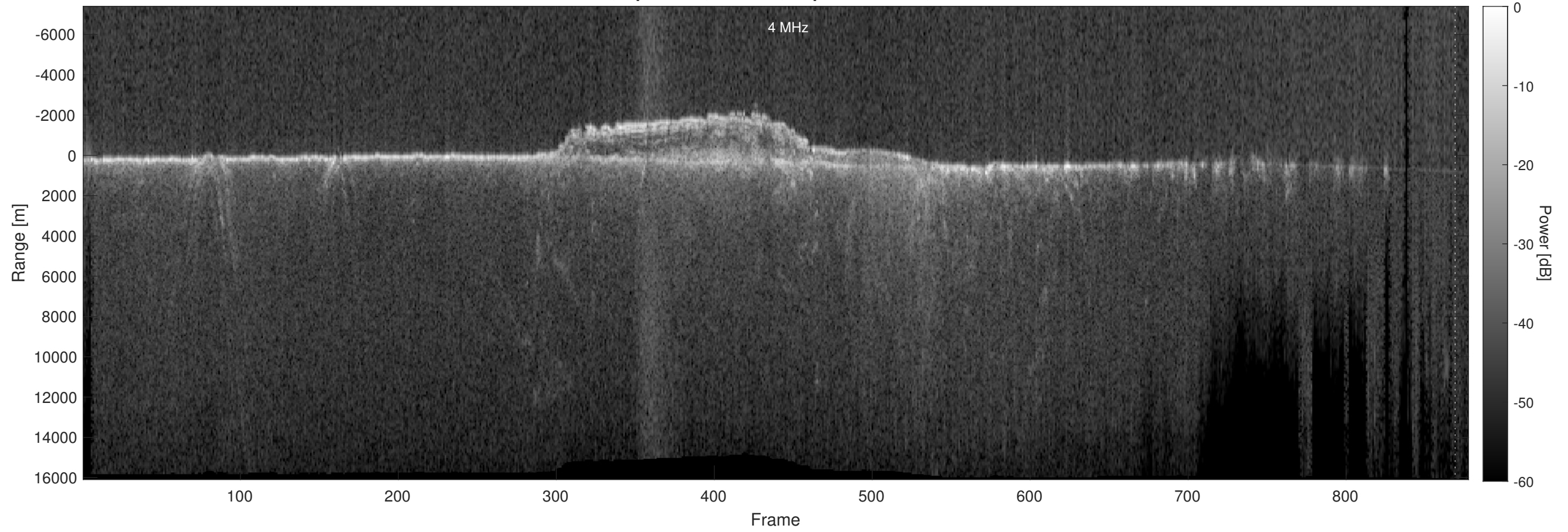
Orbit 9690, Optimized, Window, Depth-Corrected, Channel 2
