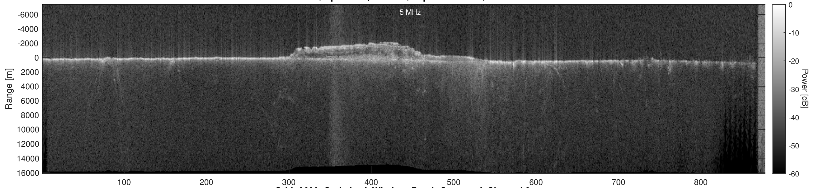
Orbit 9690, Optimized, Window, Depth-Corrected, Channel 2
