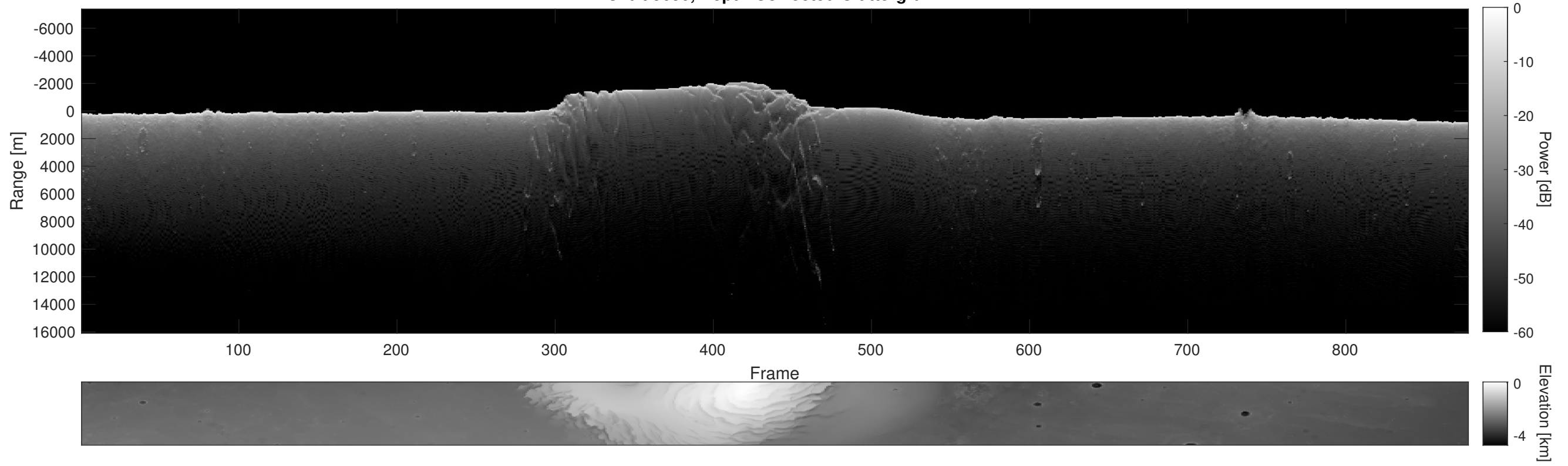
Orbit 9690, Depth-Corrected Cluttergram
