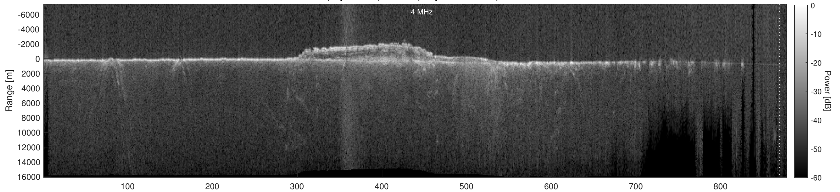
Orbit 9690, Depth-Corrected Cluttergram
