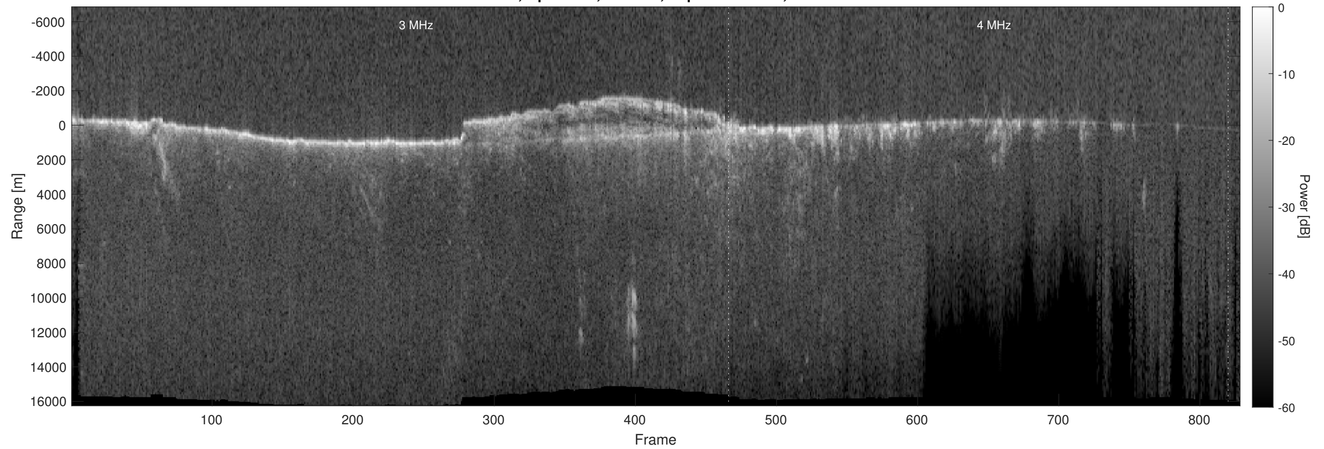
Orbit 9691, Optimized, Window, Depth-Corrected, Channel 2
