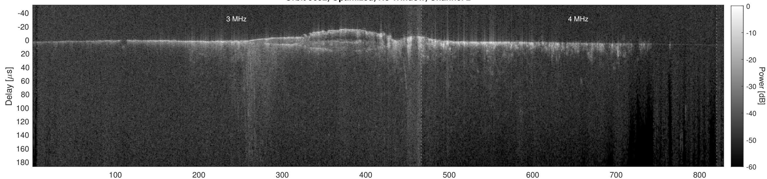
Orbit 9692, Cluttergram
